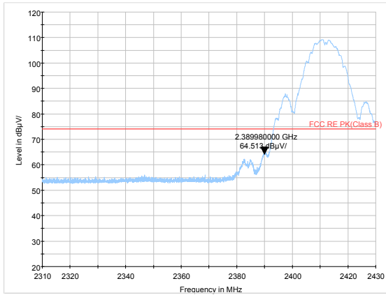
802.11b-Channel 1 Peak
