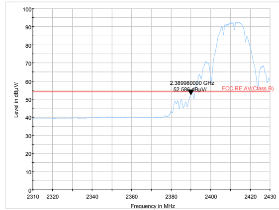
802.11b-Channel 1 Average
