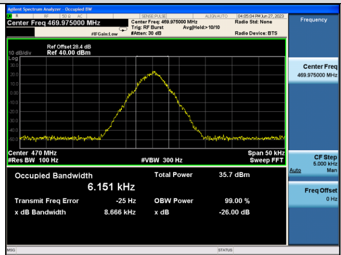
12.5kHz, 4FSK Modulation:469.975MHz-1W
