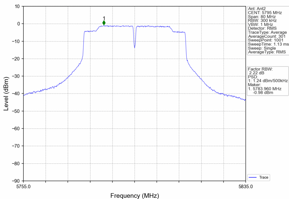
802.11ac(VHT40)_HCH_5795MHz_MIMO_NTNV
