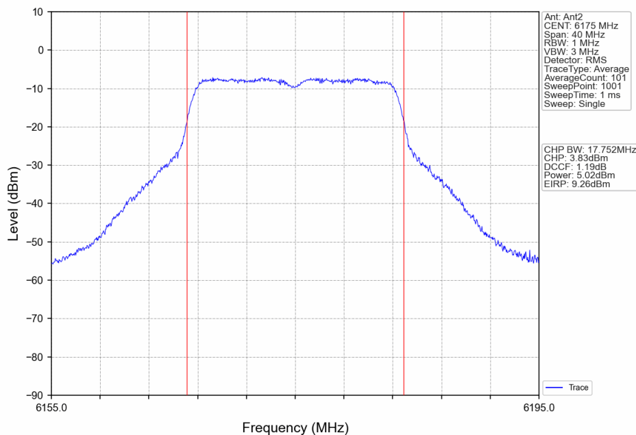
802.11ax(HEW20)_MCH_6175MHz_RU242_Left_Ant2_NTNV
