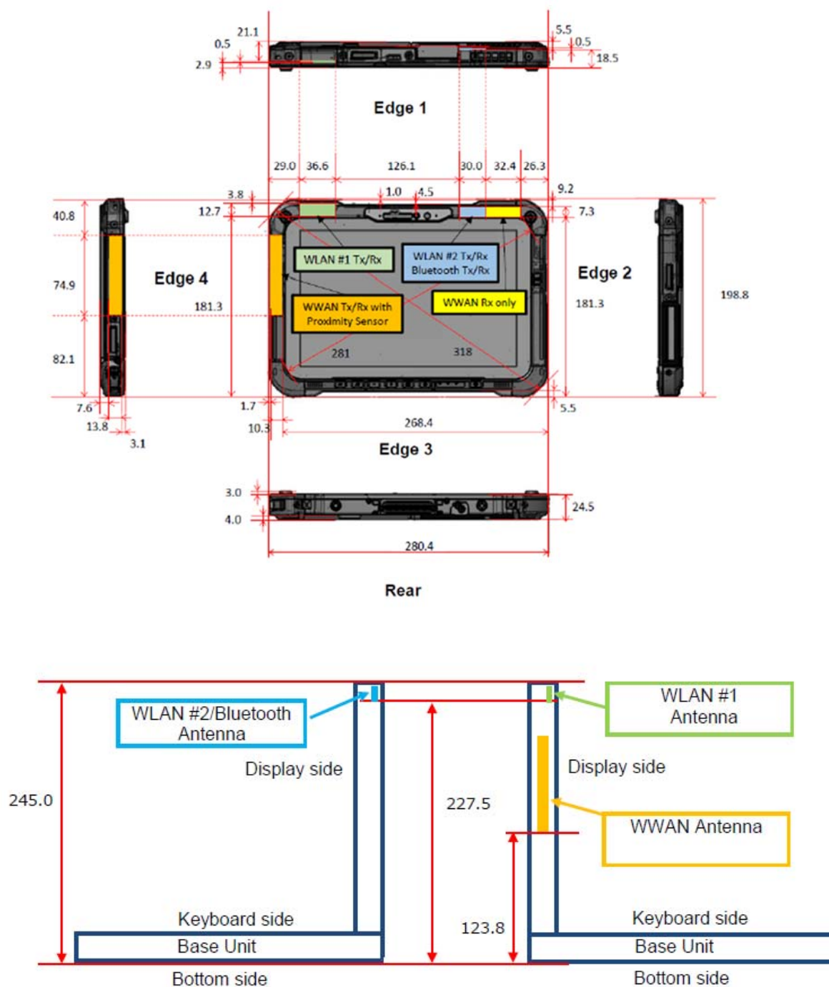
Fig2-4, Size of the device (Tablet mode)
