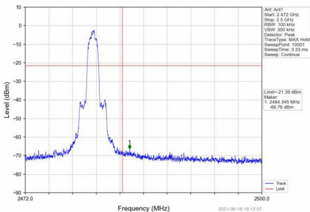
8DPSK_3DH5_HCH_2480MHz_Ant1_NTNV
