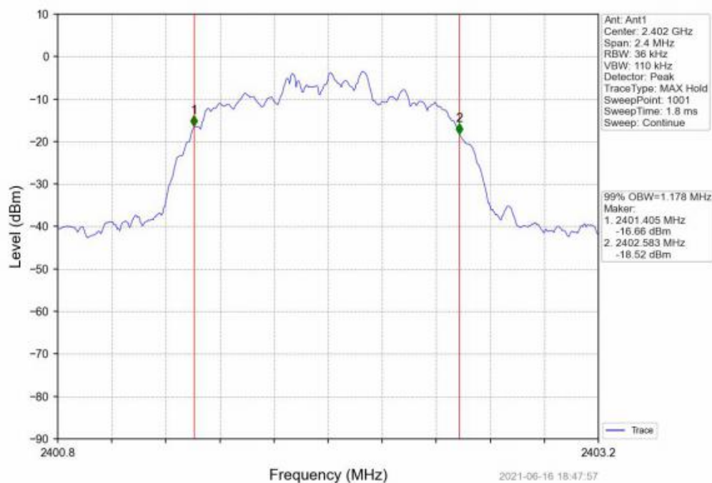
Pi/4DQPSK_2DH5_LCH_2402MHz_Ant1_NTNV
