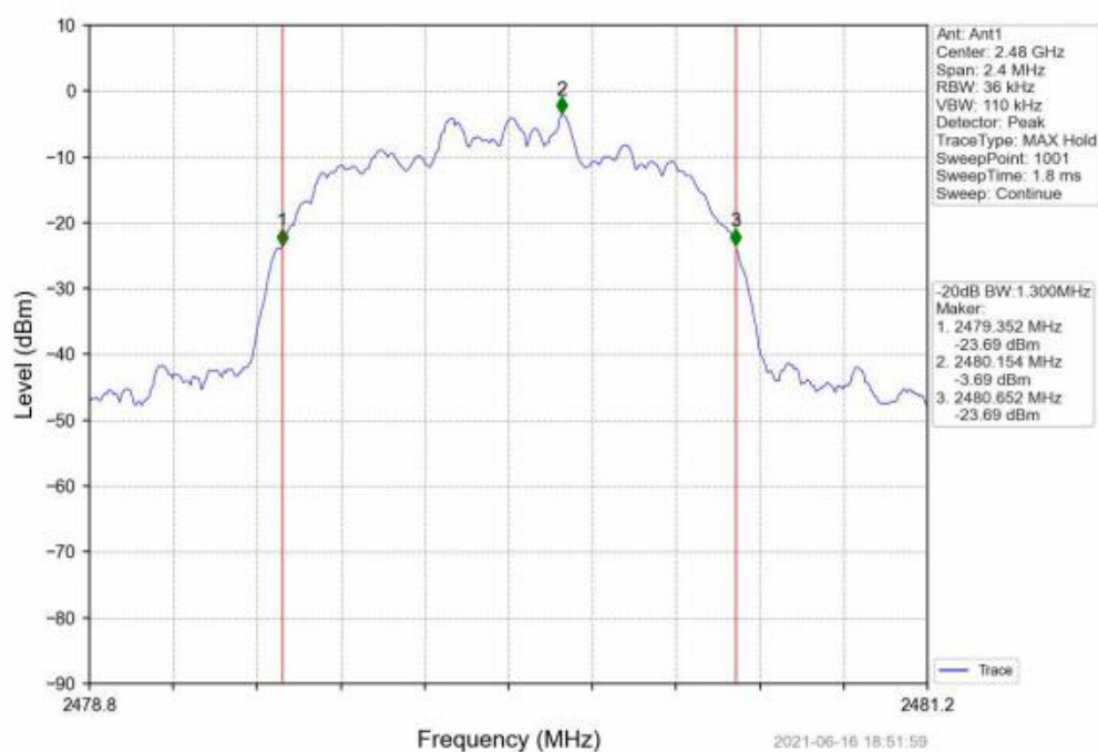
Pi/4DQPSK_2DH5_HCH_2480MHz_Ant1_NTNV
