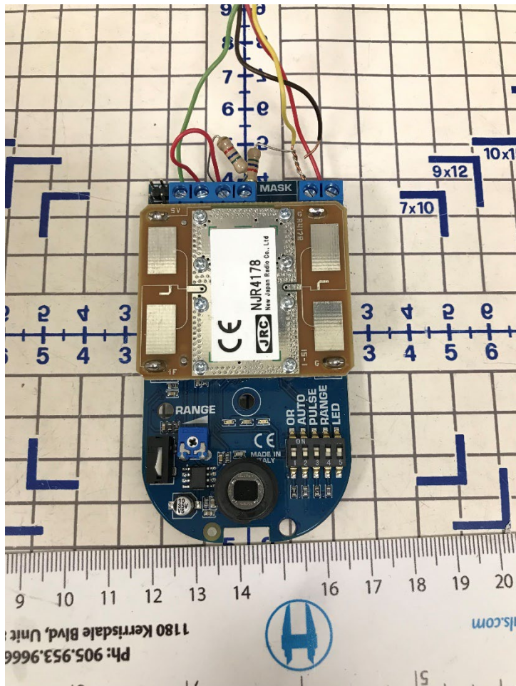
LC-204 Internal view: PCB top side view
