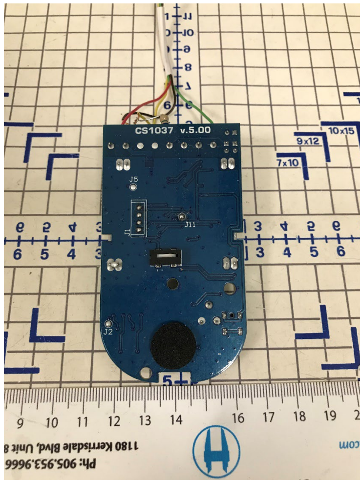
LC-204 Internal view: PCB bottom side view
