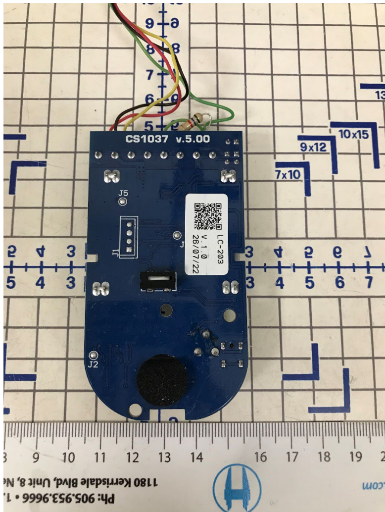
LC-203 Internal view: PCB bottom side view
