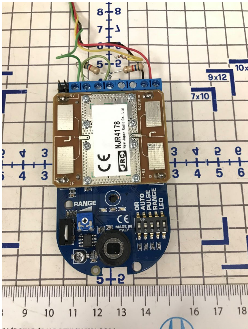
LC-203 Internal view: PCB top side view
