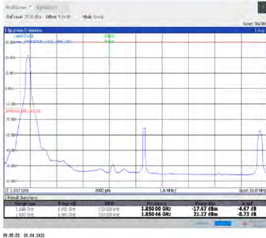
1-N25--15-15-L-1-DFT-PI2BPSK-Edge_1RB_Left-1@0-Ant1-seegraph-PASS-see graph
