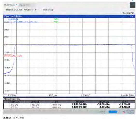
1-N25--15-15-L-6-CP-QPSK-Outer_Full-79@0-Ant1-seegraph-PASS-see graph
