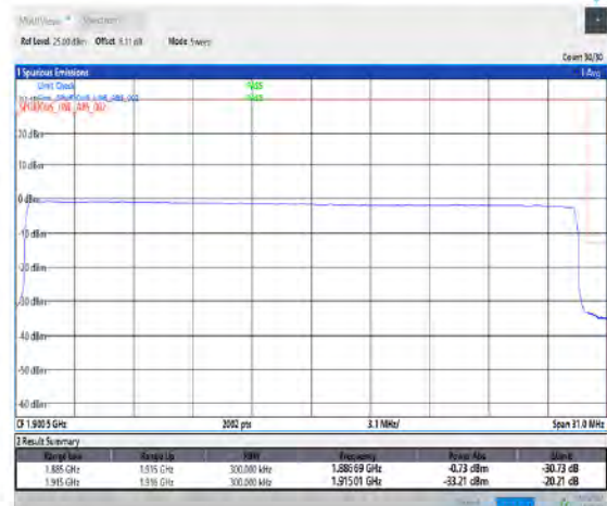
1-N25--15-30-H-6-CP-QPSK-Outer_Full-160@0-Ant1-seegraph-PASS-see graph
