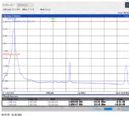
1-N25--15-15-L-4-CP-QPSK-Edge_1RB_Left-1@0-Ant1-seegraph-PASS-see graph
