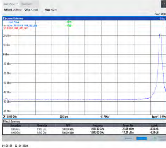
1-N25-15-40-H-2-DFT-PI2BPSK-Edge_1RB_Right-1@215-Ant1-seegraph-PASS-see graph
