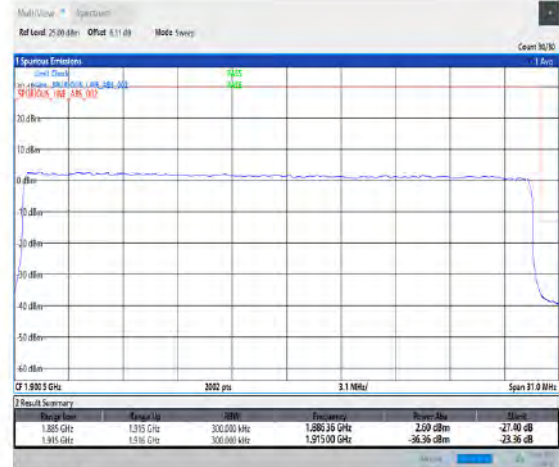
1-N25--15-30-H-3-DFT-PI2BPSK-Outer_Full-160@0-Ant1-seegraph-PASS-see graph
