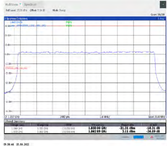
1-N25--15-15-L-3-DFT-PI2BPSK-Outer_Full-75@0-Ant1-seegraph-PASS-see graph
