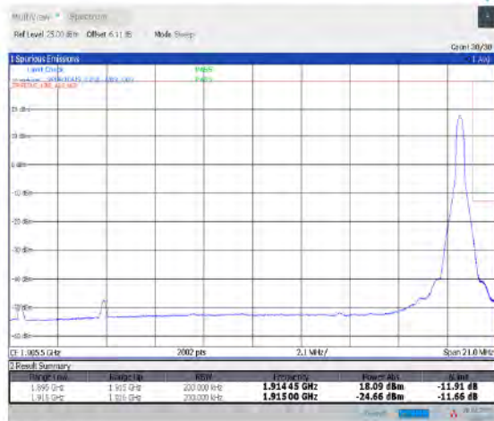
1-N25-15-20-H-5-CP-QPSK-Edge_1RB_Right-1@105-Ant1-seegraph-PASS-see graph
