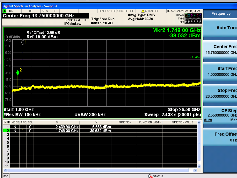
BLE_1M-Ant1-2440-1000~26500-PASS
