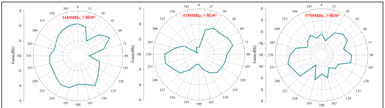
Ant2
