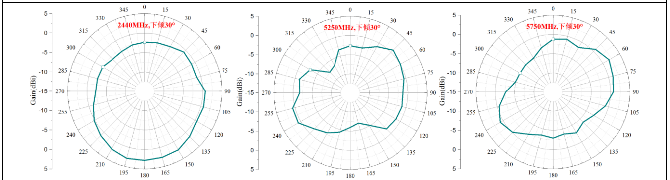
Ant3
