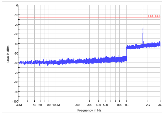
LTE Band 4 3MHzCH-Middle 30MHz~3GHz
