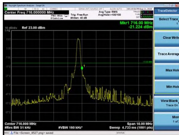
LTE Band 12 16QAM 1.4MHz CH-High, 1 RB
