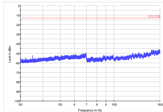
LTE Band 4 3MHzCH-High 3GHz~18GHz
