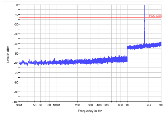
LTE Band 4 3MHzCH-High 30MHz~3GHz
