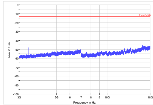
LTE Band 4 3MHzCH-Middle 3GHz~18GHz
