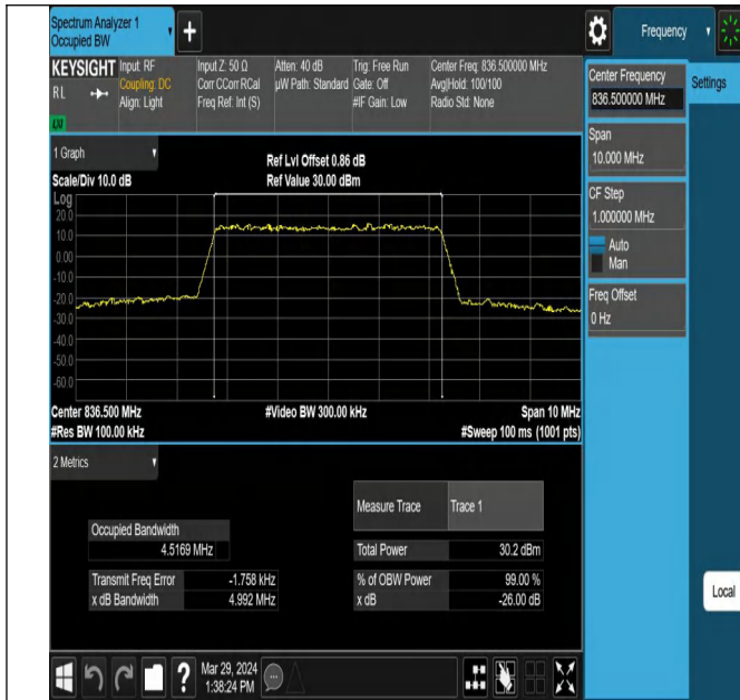
Band5-5MHz-QPSK-20525-25RB#0-PASS
