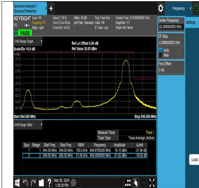
Band5_5MHz_QPSK_20625_1RB#24
