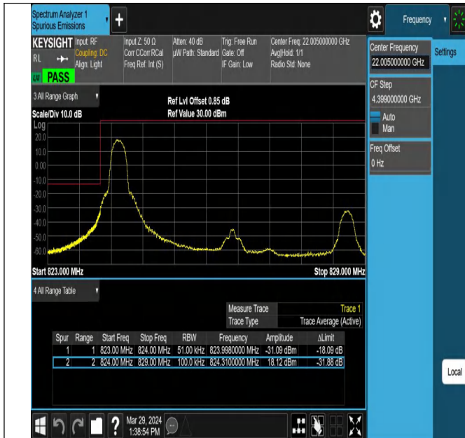
Band5_5MHz_QPSK_20425_1RB#0
