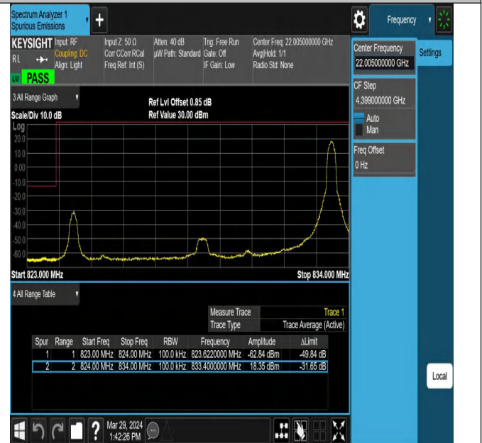
Band5_10MHz_QPSK_20450_1RB#49
