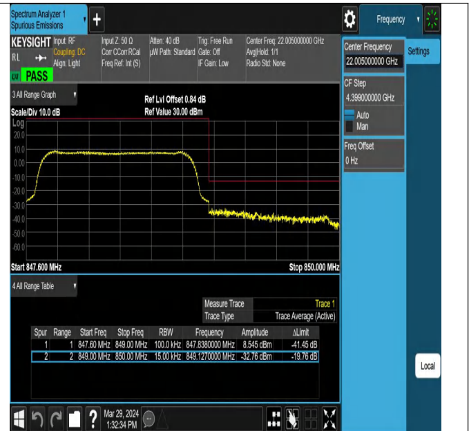
Band5_1.4MHz_QPSK_20643_6RB#0
