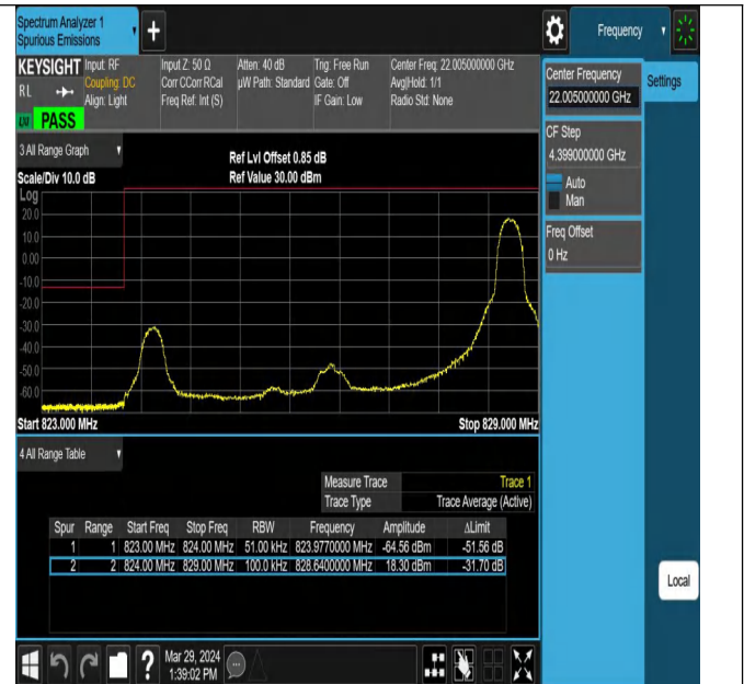
Band5_5MHz_QPSK_20425_1RB#24
