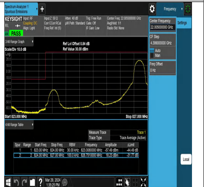
Band5_3MHz_QPSK_20415_1RB#14
