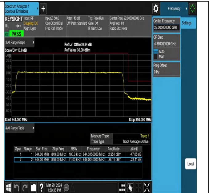
Band5_5MHz_QPSK_20625_25RB#0
