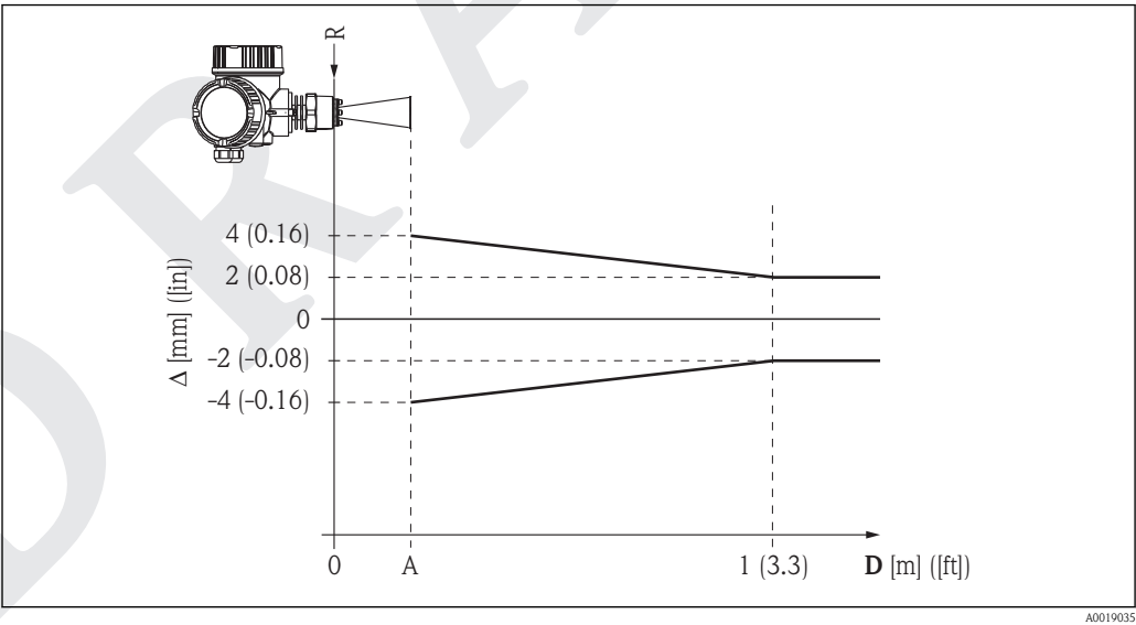
11 Maximum measured error in near-range applications; values for standard version
