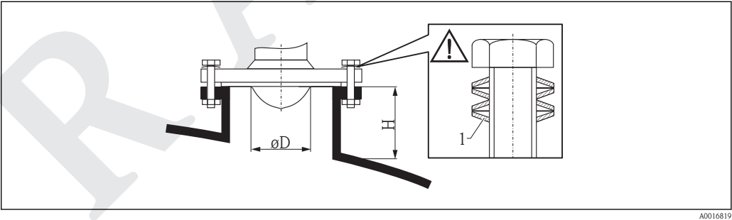
15 Nozzle height and diameter for horn antenna, flush mount (FMR52)
