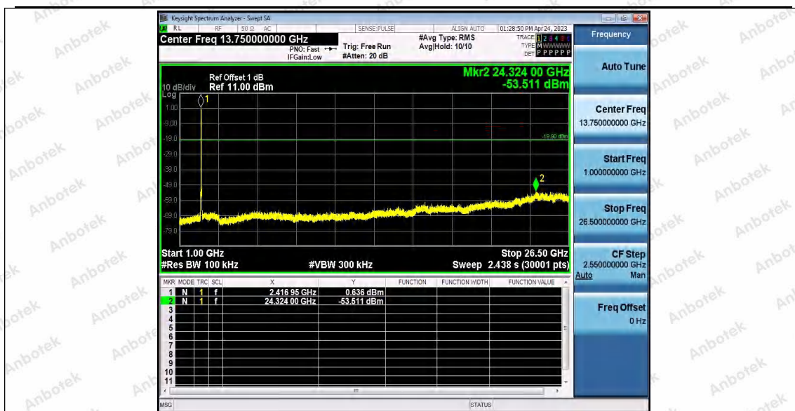
11N40SISO_Ant2_2422_0~Reference
