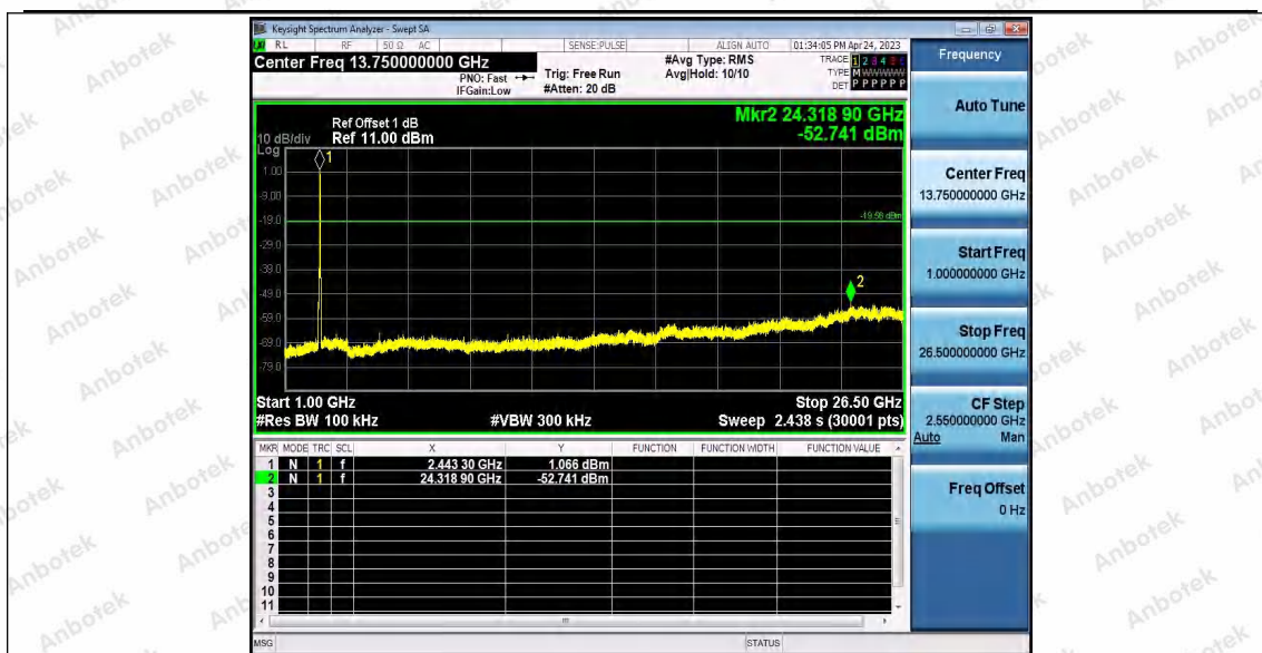
11N40SISO_Ant2_2452_0~Reference
