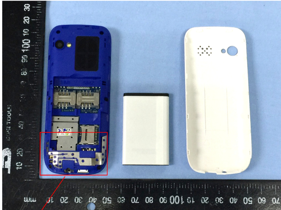
2G Antenna
