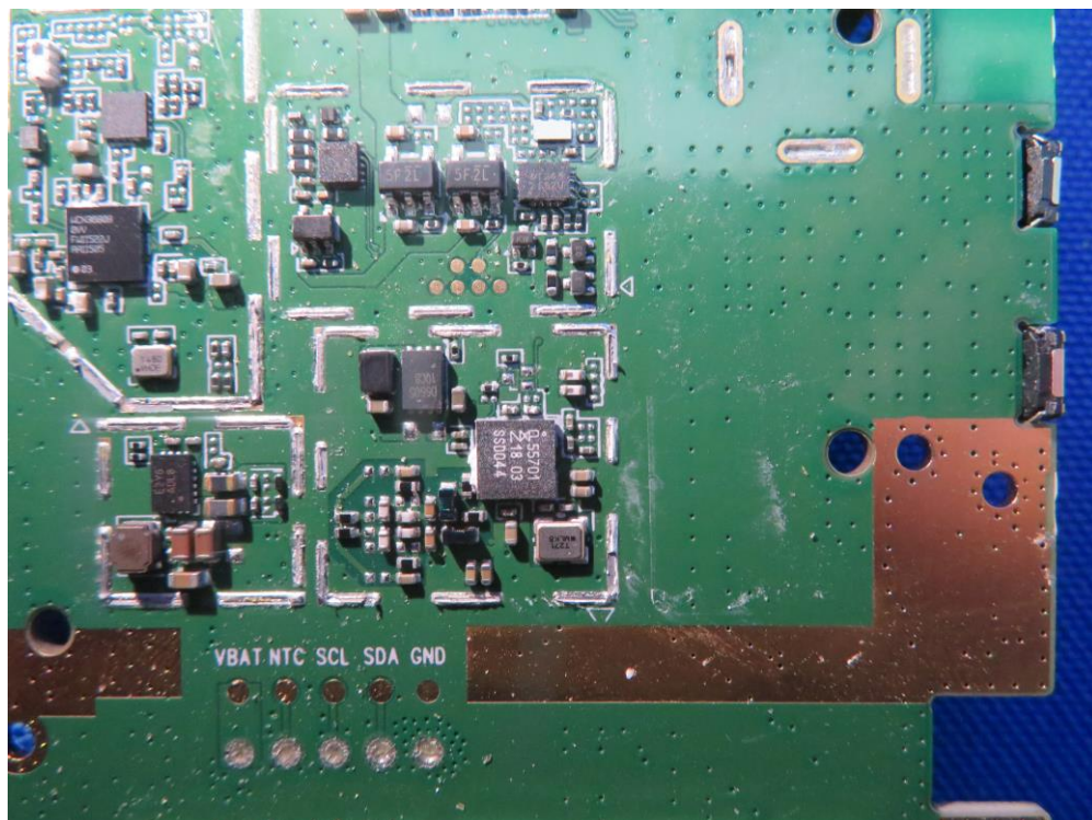
(16) EUT Photo (PN557 NFC chipset)
