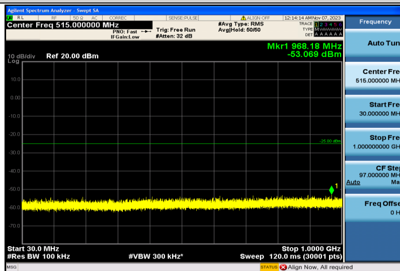
Band7-10MHz-16QAM-21100-1RB#0-30~1000MHz
