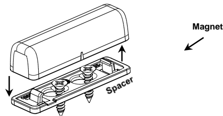
Fig. 5 – Magnet Mounting
