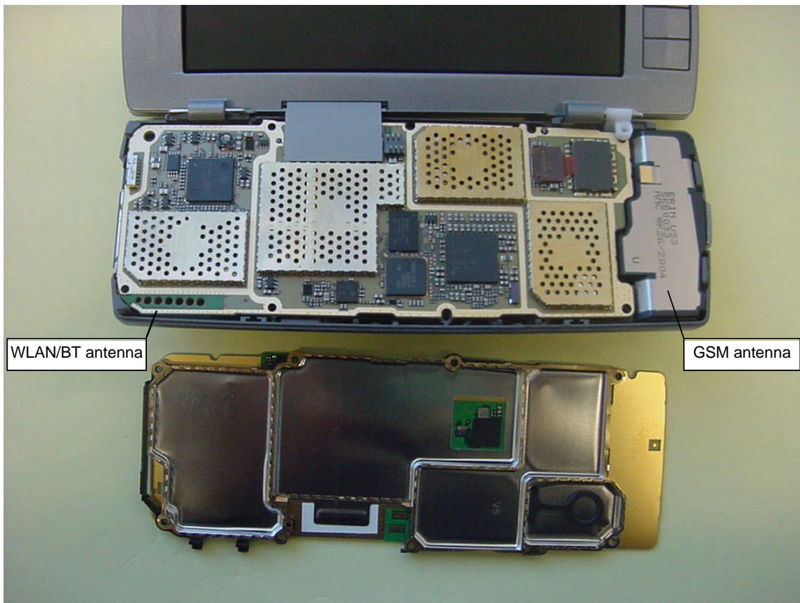
Picture 1. Antenna locations
