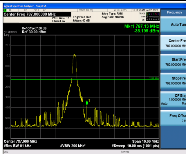
Band13-5MHz-QPSK-23255-1-5-High--38.20-PASS
