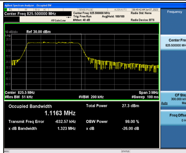
Band5-3MHz-16QAM-20415-6-0-Low-1.1163-1.323-PASS
