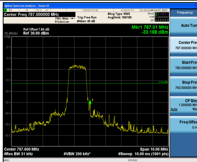
Band13-5MHz-QPSK-23255-6-0-High--33.17-PASS
