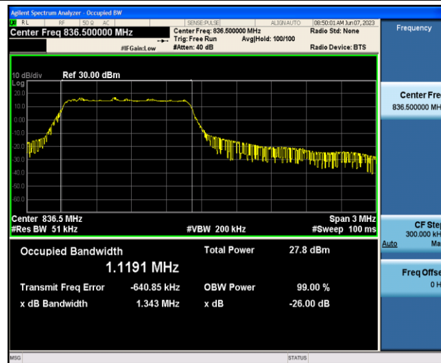
Band5-3MHz-QPSK-20525-6-0-Low-1.1191-1.343-PASS
