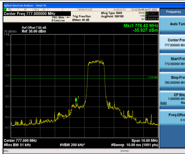
Band13-5MHz-QPSK-23205-6-0-Low--35.93-PASS
