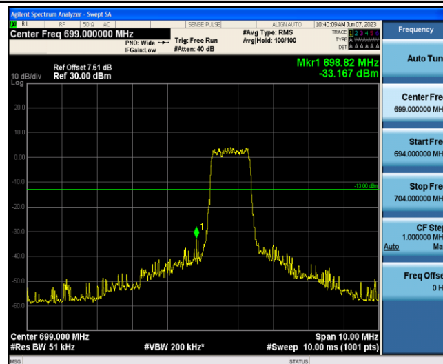
Band12-5MHz-QPSK-23035-6-0-Low--33.17-PASS
