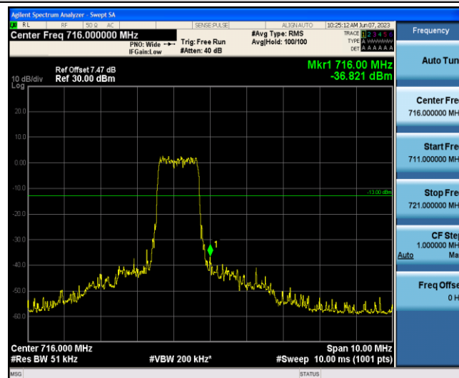
Band12-3MHz-QPSK-23165-6-0-High--36.82-PASS
