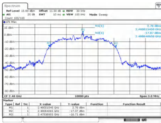
8DPSK_3-DH5_Channel 78
