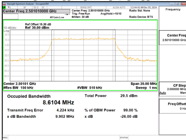
Band41_10MHz_DFT_s_OFDM_SCS30kHz_64QAM_RB24_0_CH500202
