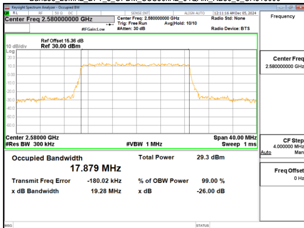
Band38_20MHz_DFT_s_OFDM_SCS30kHz_64QAM_RB50_0_CH516000
