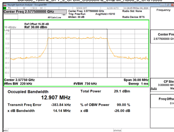
Band38_15MHz_DFT_s_OFDM_SCS30kHz_64QAM_RB36_0_CH515500
