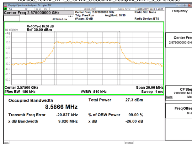
Band38_10MHz_DFT_s_OFDM_SCS30kHz_256QAM_RB24_0_CH515000
