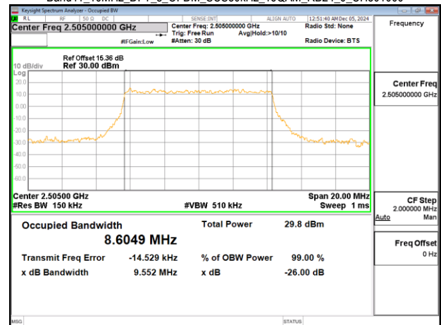
Band41_10MHz_DFT_s_OFDM_SCS30kHz_16QAM_RB24_0_CH501000
