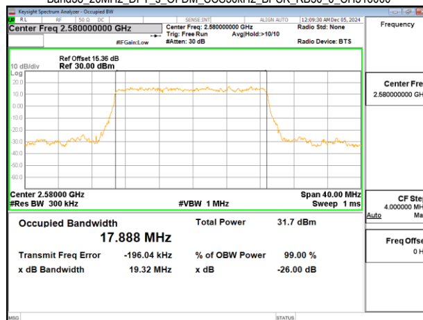
Band38_20MHz_DFT_s_OFDM_SCS30kHz_BPSK_RB50_0_CH516000
