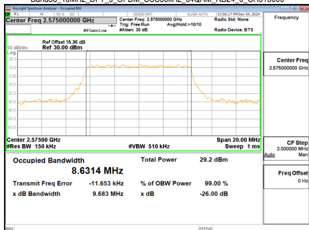
Band38_10MHz_DFT_s_OFDM_SCS30kHz_64QAM_RB24_0_CH515000
