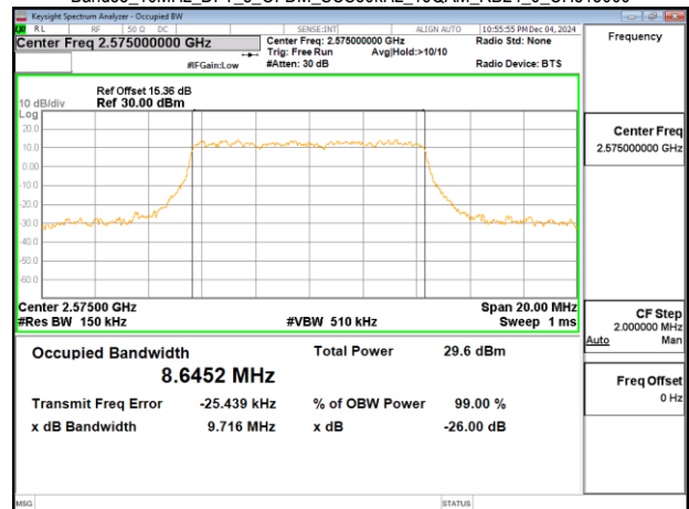
Band38_10MHz_DFT_s_OFDM_SCS30kHz_16QAM_RB24_0_CH515000
