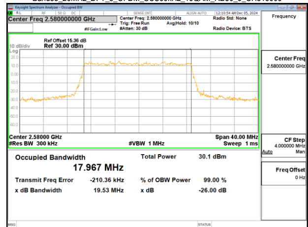
Band38_20MHz_DFT_s_OFDM_SCS30kHz_16QAM_RB50_0_CH516000
