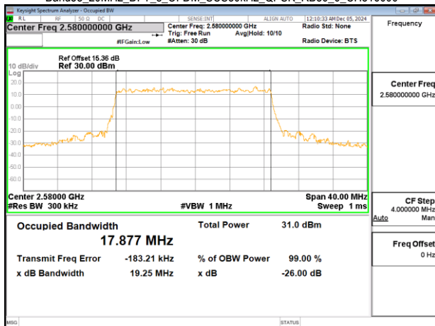
Band38_20MHz_DFT_s_OFDM_SCS30kHz_QPSK_RB50_0_CH516000
