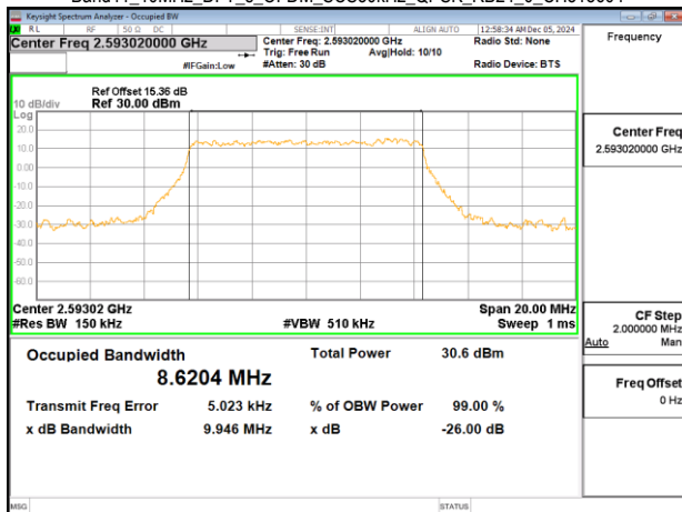
Band41_10MHz_DFT_s_OFDM_SCS30kHz_QPSK_RB24_0_CH518604
