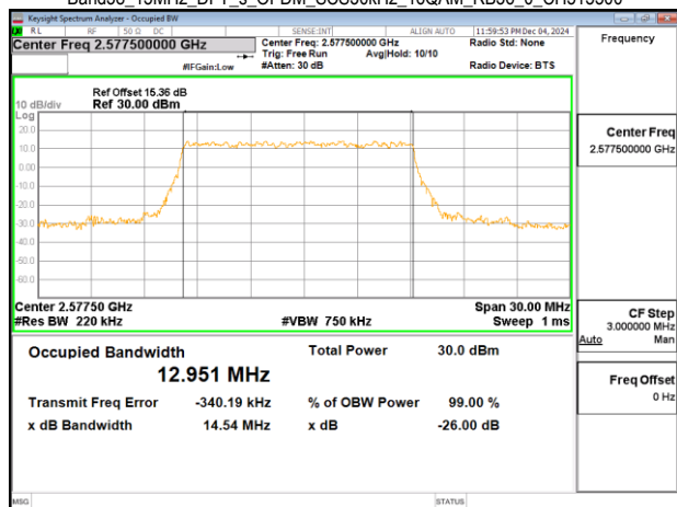
Band38_15MHz_DFT_s_OFDM_SCS30kHz_16QAM_RB36_0_CH515500
