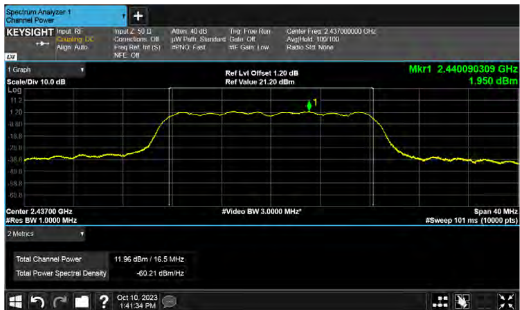
802.11g CH6
