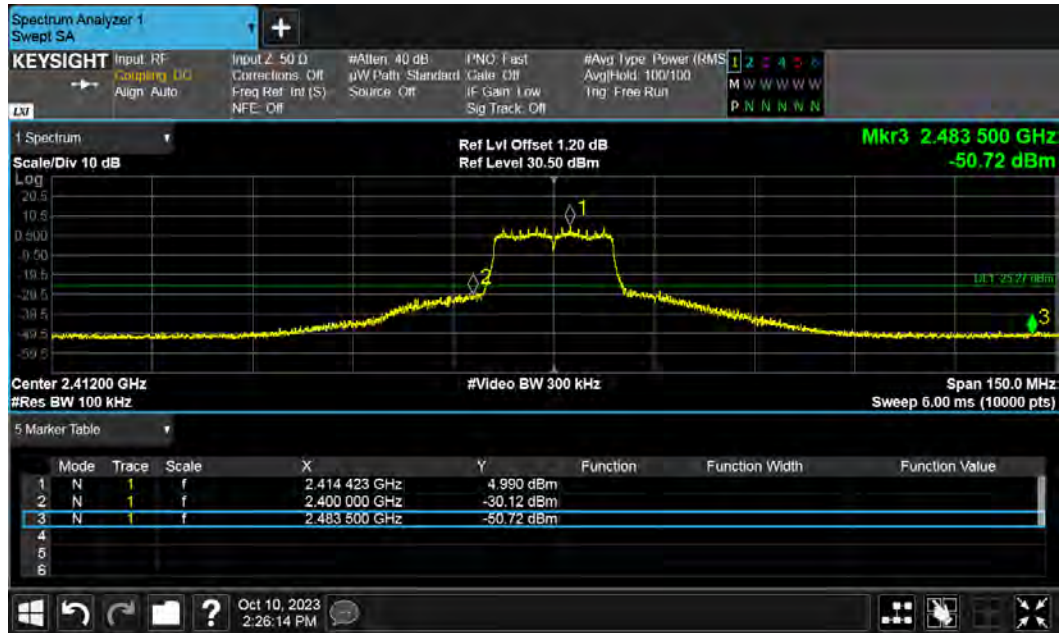
802.11n_Conducted Band Edge – 2412 MHz
