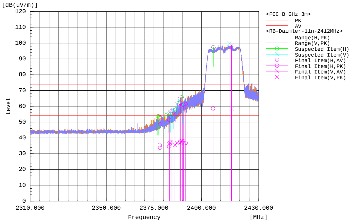
Band-Edge 802.11n - 2412 MHz
