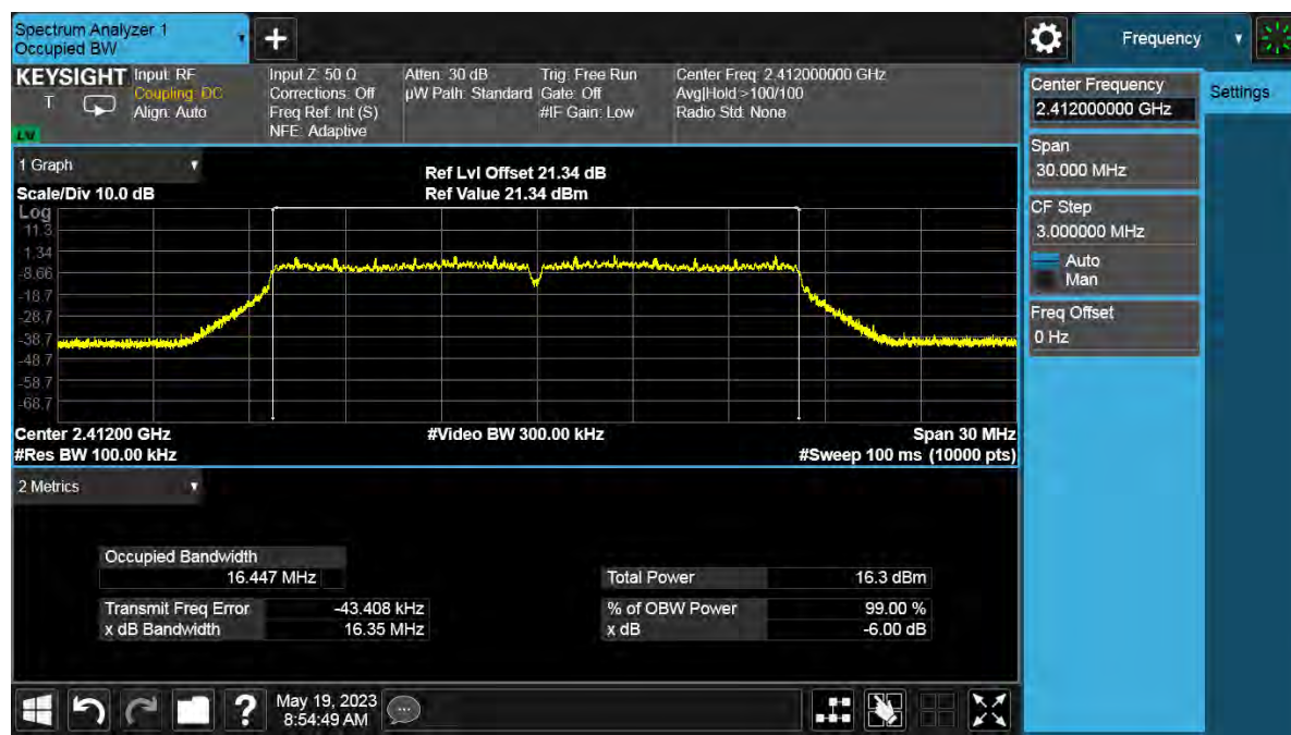
DTS BW at 802.11g CH1
