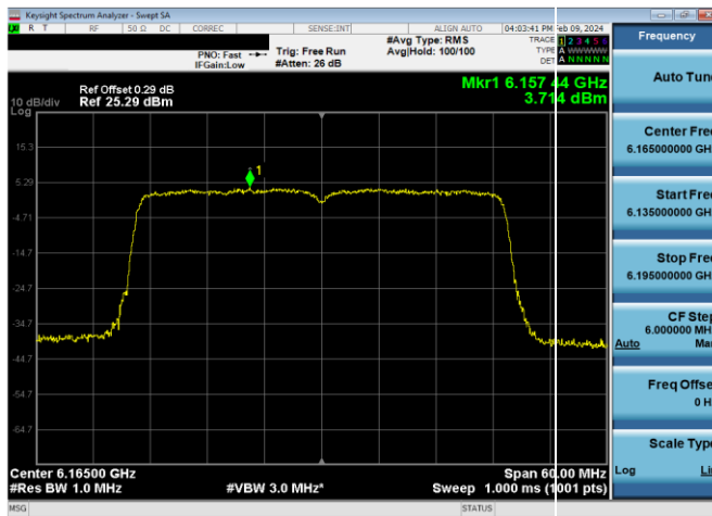
Plot 7-353. Power Spectral Density Plot Antenna 4a Standard Power (40MHz 802.11ax (UNII Band 5) – Ch. 43, MCS11)
