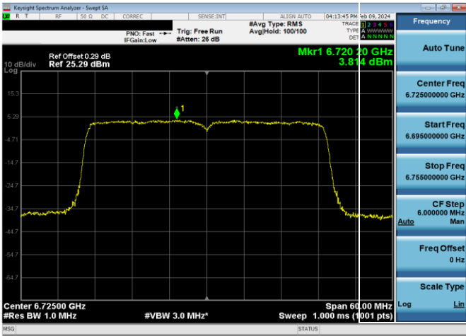
Plot 7-358. Power Spectral Density Plot Antenna 4a Standard Power (40MHz 802.11ax (UNII Band 7) – Ch. 155, MCS11)
