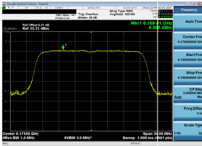
Plot 7-352. Power Spectral Density Plot Antenna 4a Standard Power (20MHz 802.11ax (UNII Band 5) – Ch. 45, MCS11)
