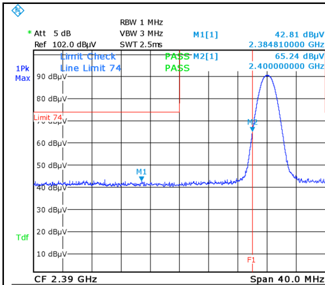
GFSK-Left Side-PK
