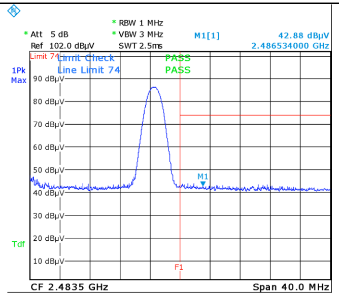
GFSK-Right Side-PK
