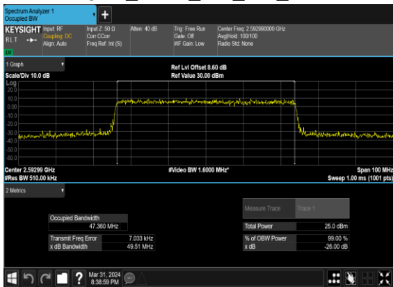
N41(50M)_CP-OFDM_256 QAM_Outer_Full_Mid_CH
