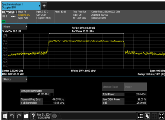
N41(50M)_CP-OFDM_16 QAM_Outer_Full_Mid_CH
