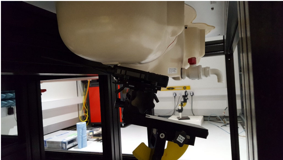
Figure 95 Right Tilt - 1160 mAh Battery (Part no: 300-01852) 1/4 Wave Whip Antenna (Part no: 310-00015)
