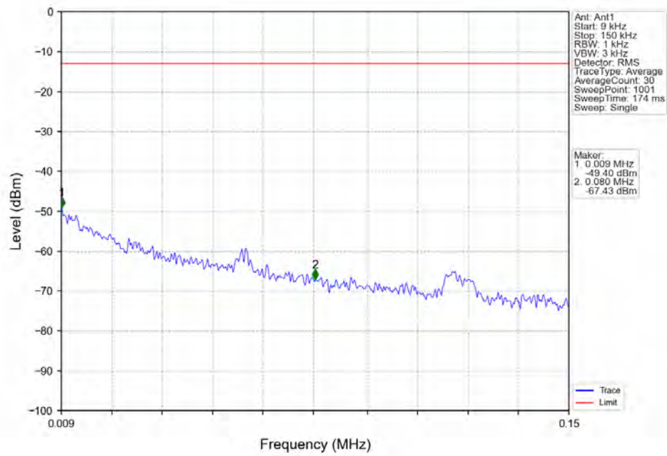
Band26a 1.4MHz 16QAM HCH 823.3MHz RB 1 0 NTN
