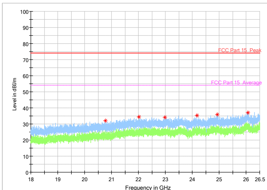
Fig. 37 Radiated Spurious Emission (802.11a, ch52, 18 GHz-26.5 GHz)
