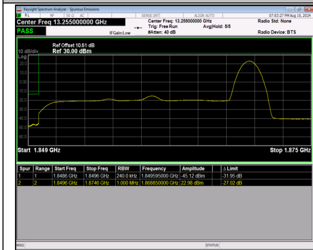
2-2-20MHz-5MHz-QPSK@QPSK-QPSK@QPSK-18700-1 8817-1RB#99@100RB#0-0RB#0@25RB#0-PASS
