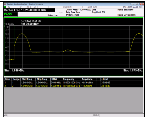
2-2-20MHz-5MHz-QPSK@QPSK-QPSK@QPSK-18700-18 817-1RB#0@100RB#0-1RB#24@25RB#0-PASS
