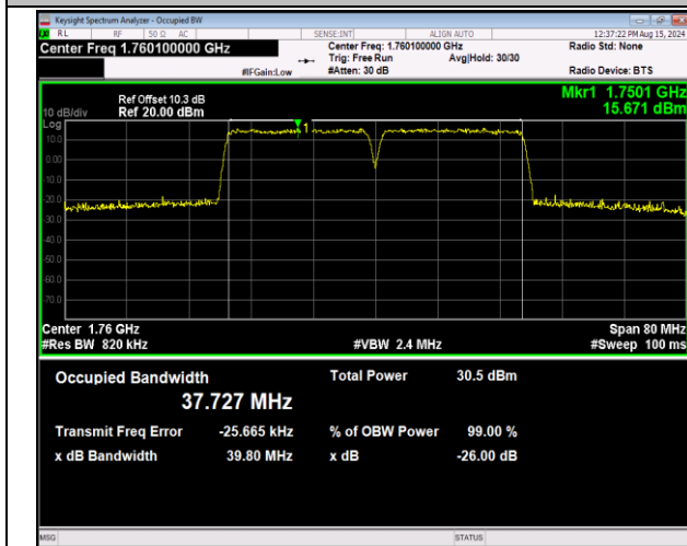
66-66-20MHz-20MHz-16QAM-16QAM-132374-132572-10 ORB#0-100RB#0-PASS
