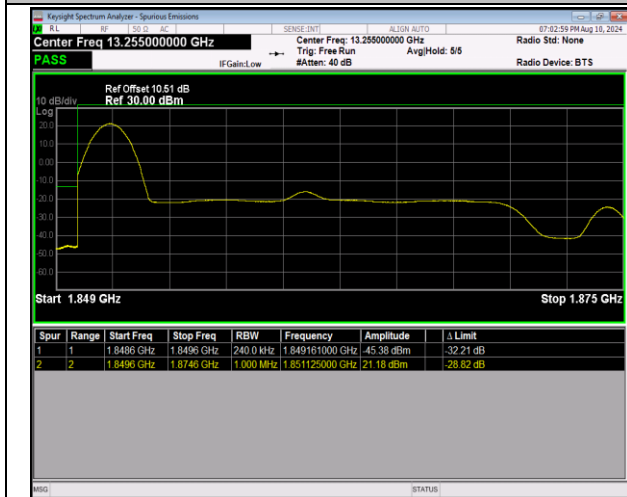
2-2-20MHz-5MHz-16QAM@16QAM-16QAM@16QAM-18 700-18817-1RB#0@100RB#0-0RB#0@25RB#0-PASS
