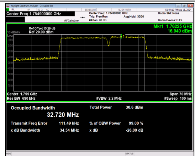
66-66-20MHz-15MHz-64QAM-64QAM-132348-132519-10 ORB#0-75RB#0-PASS
