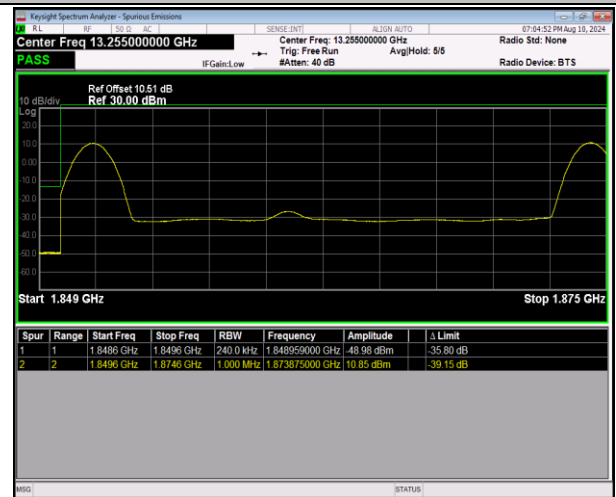
2-2-20MHz-5MHz-16QAM@16QAM-16QAM@16QAM-187 00-18817-1RB#0@100RB#0-1RB#24@25RB#0-PASS
