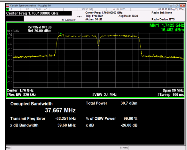
66-66-20MHz-20MHz-64QAM-64QAM-132374-132572-10 ORB#0-100RB#0-PASS
