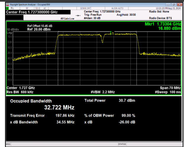
66-66-20MHz-15MHz-16QAM-16QAM-132072-132243-10 ORB#0-75RB#0-PASS
