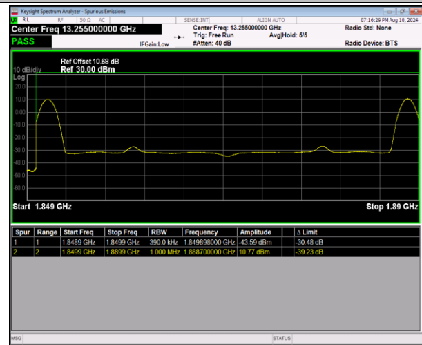
2-2-20MHz-20MHz-16QAM@16QAM-16QAM@16QAM-18700-18898-1RB#0@100RB#0-1RB#99@100RB#0-PASS
