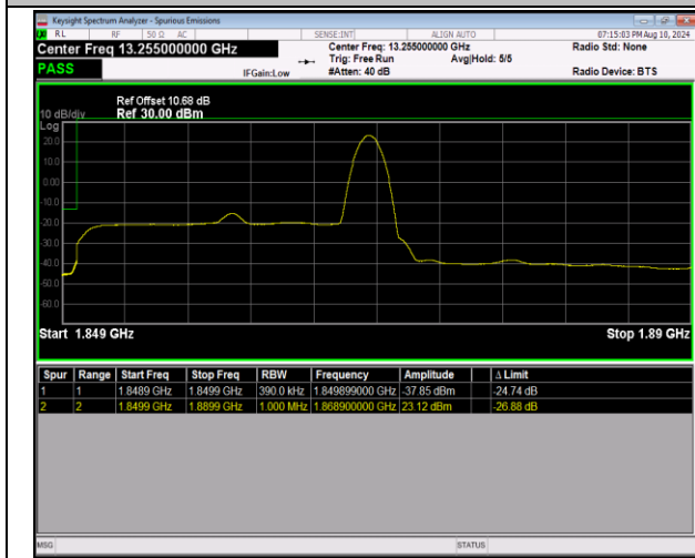
2-2-20MHz-20MHz-QPSK@QPSK-QPSK@QPSK-18700-18898-1RB#99@100RB#0-0RB#0@100RB#0-PASS
