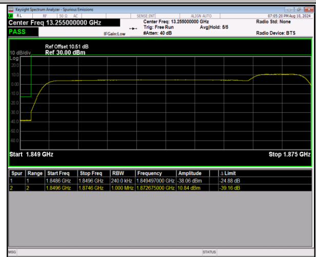
2-2-20MHz-5MHz-QPSK@QPSK-QPSK@QPSK-18700-18 817-100RB#0@100RB#0-25RB#0@25RB#0-PASS
