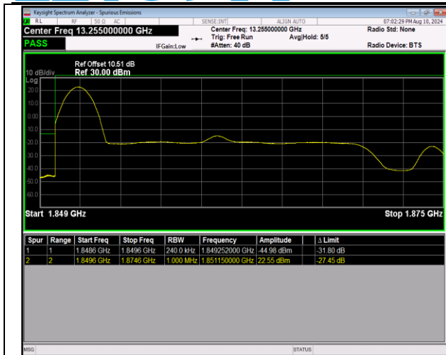
2-2-20MHz-5MHz-QPSK@QPSK-QPSK@QPSK-18700-1 8817-1RB#0@100RB#0-0RB#0@25RB#0-PASS
