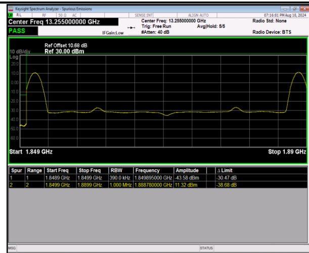
2-2-20MHz-20MHz-QPSK@QPSK-QPSK@QPSK-18700-18898-1RB#0@100RB#0-1RB#99@100RB#0-PASS
