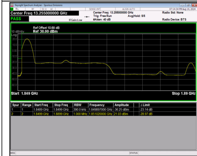
2-2-20MHz-20MHz-16QAM@16QAM-16QAM@16QAM-18700-18898-1RB#0@100RB#0-0RB#0@100RB#0-PASS
