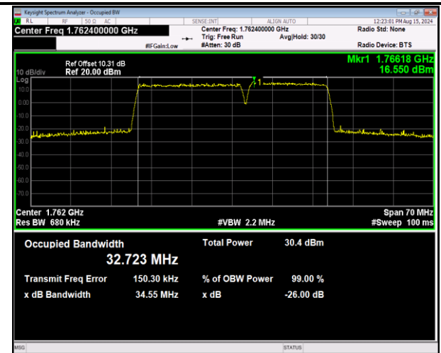
66-66-20MHz-15MHz-16QAM-16QAM-132423-132594-10 ORB#0-75RB#0-PASS
