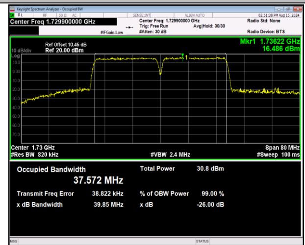
66-66-20MHz-20MHz-64QAM-64QAM-132072-132270-10 ORB#0-100RB#0-PASS
