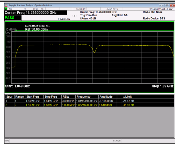
2-2-20MHz-20MHz-QPSK@QPSK-QPSK@QPSK-18700-18898-100RB#0@100RB#0-100RB#0@100RB#0-PASS
