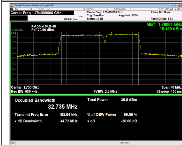
66-66-20MHz-15MHz-16QAM-16QAM-132348-132519-10 ORB#0-75RB#0-PASS
