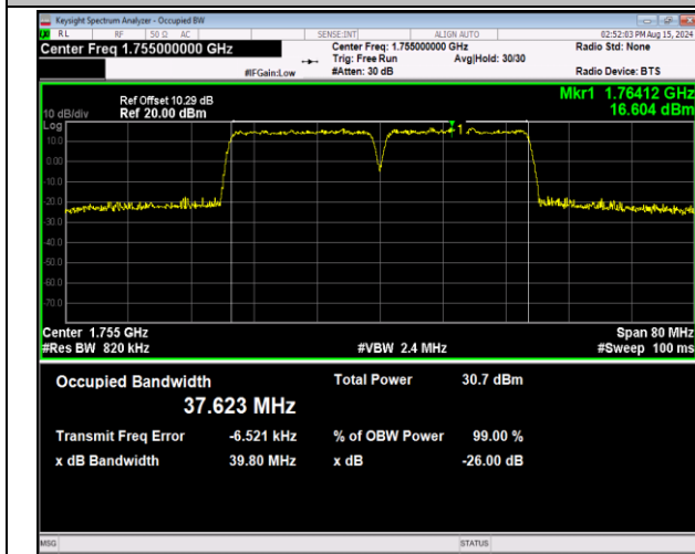
66-66-20MHz-20MHz-64QAM-64QAM-132323-132521-10 ORB#0-100RB#0-PASS
