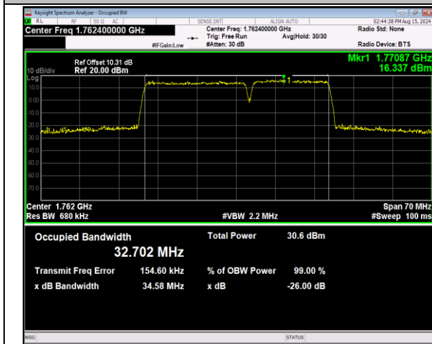
66-66-20MHz-15MHz-64QAM-64QAM-132423-132594-10 ORB#0-75RB#0-PASS
