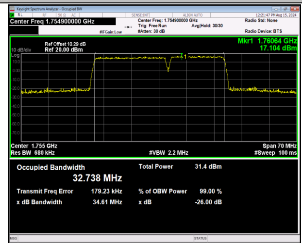
66-66-20MHz-15MHz-QPSK-QPSK-132348-132519-100R B#0-75RB#0-PASS
