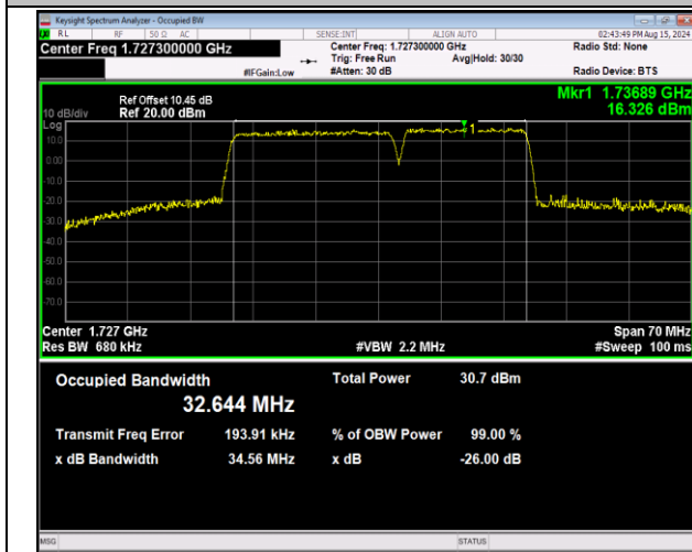
66-66-20MHz-15MHz-64QAM-64QAM-132072-132243-10 ORB#0-75RB#0-PASS
