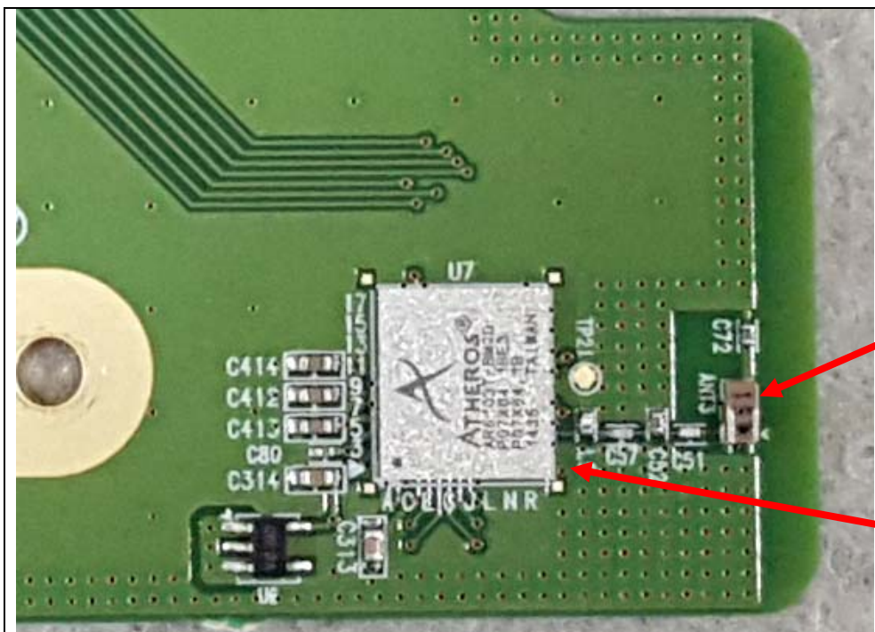
WiFi Antenna
