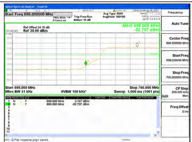
Band12 / 5MHz / Low CH / QPSK / FULL RB
