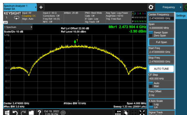
CH34 (2474MHz)
