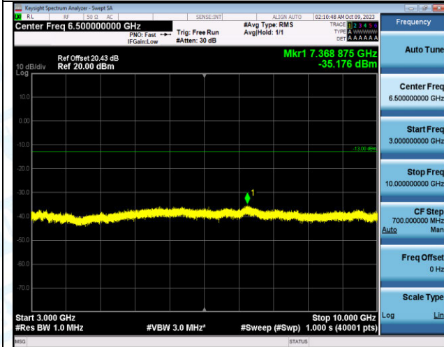
Band12_3MHz_QPSK_23025_15RB#0_3000~10000_3000~10000 0~10000
