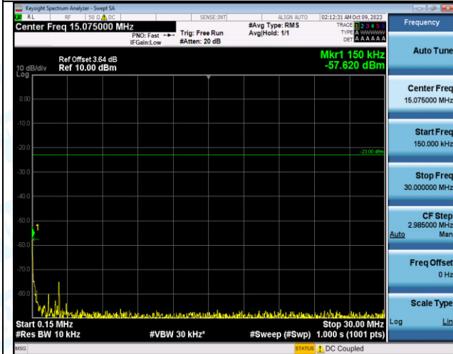
Band12_3MHz_16QAM_23095_1RB#0_0.15~30_0.15~30
