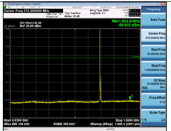
Band12_5MHz_16QAM_23035_1RB#0_30~1000_30~1000 0
