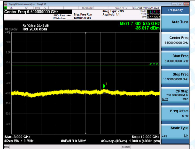
Band12_3MHz_16QAM_23165_15RB#0_3000~10000_30 00~10000
