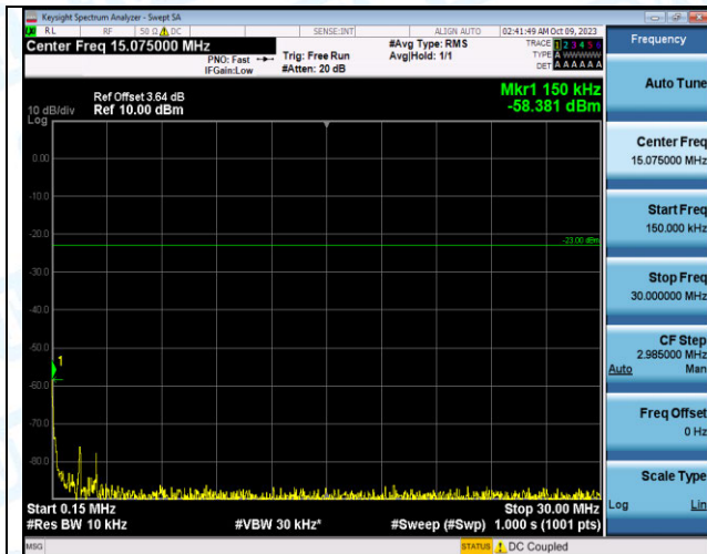
Band12_5MHz_16QAM_23035_1RB#0_0.15~30_0.15~30
