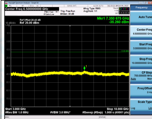
Band12_3MHz_QPSK_23165_1RB#0_3000~10000_3000~10000
