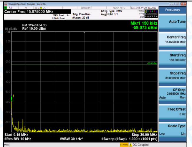
Band12_3MHz_QPSK_23095_1RB#0_0.15~30_0.15~30
