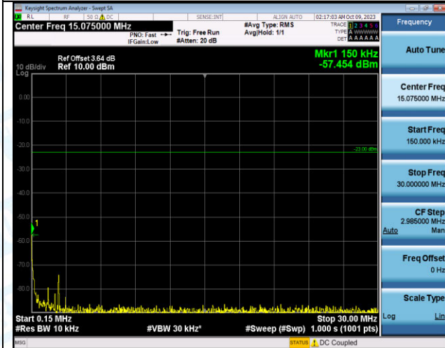
Band12_3MHz_16QAM_23165_15RB#0_0.15~30_0.15~3 0
