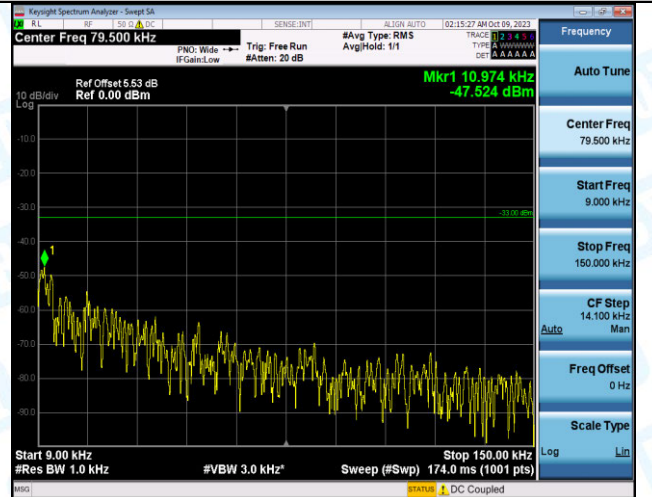
Band12_3MHz_16QAM_23165_1RB#0_0.009~0.15_0.009~0.15
