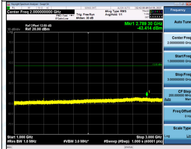
Band12_5MHz_16QAM_23035_1RB#0_1000~3000_1000~3000
