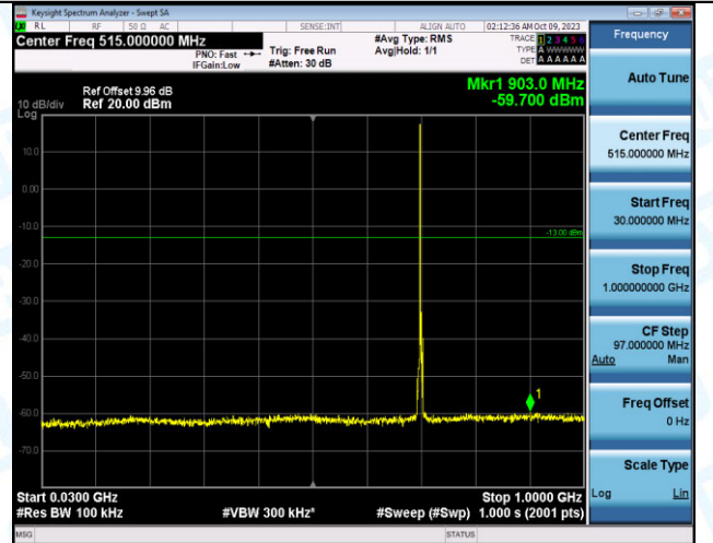
Band12_3MHz_16QAM_23095_1RB#0_30~1000_30~1000 0
