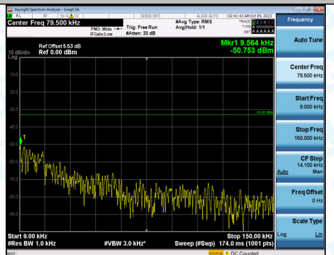
Band12_5MHz_16QAM_23035_1RB#0_0.009~0.15_0.009 ~0.15
