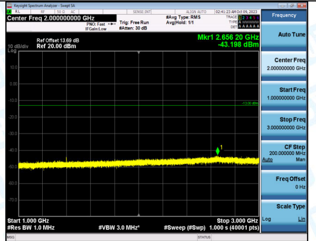
Band12_5MHz_QPSK_23035_1RB#0_1000~3000_1000~3 000
