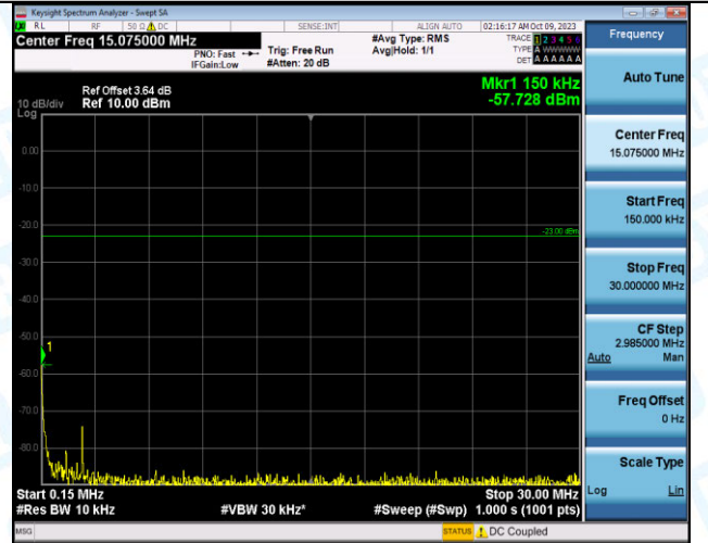
Band12_3MHz_QPSK_23165_15RB#0_0.15~30_0.15~30
