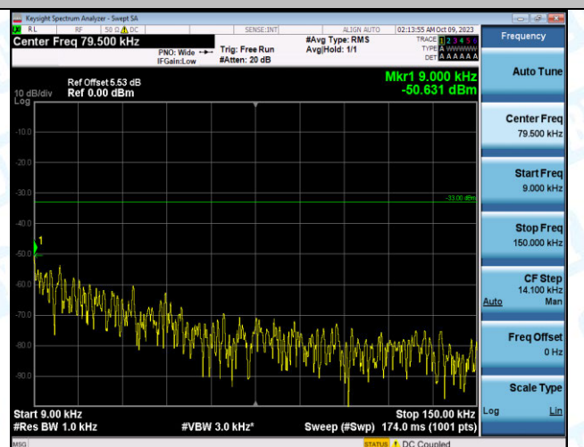
Band12_3MHz_16QAM_23095_15RB#0_0.009~0.15_0.00 9~0.15
