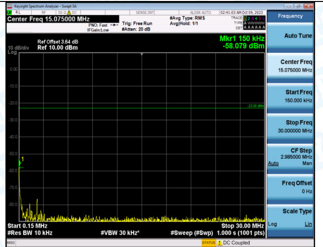
Band12_5MHz_QPSK_23035_1RB#0_0.15~30_0.15~30
