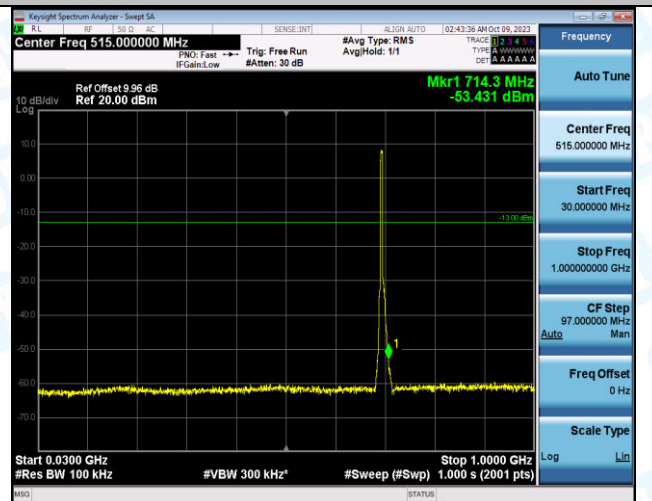
Band12_5MHz_16QAM_23035_25RB#0_30~1000_30~1000 00
