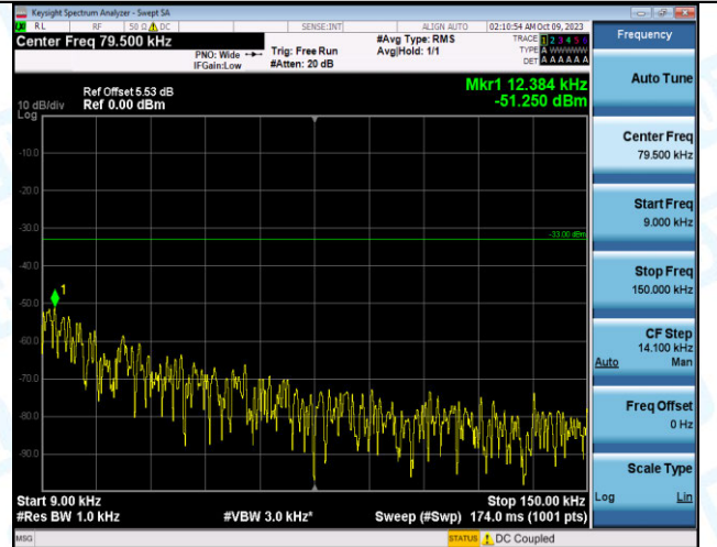
Band12_3MHz_16QAM_23025_15RB#0_0.009~0.15_0.009~0.15 9~0.15
