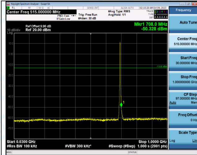
Band12_3MHz_QPSK_23025_15RB#0_30~1000_30~100 0
