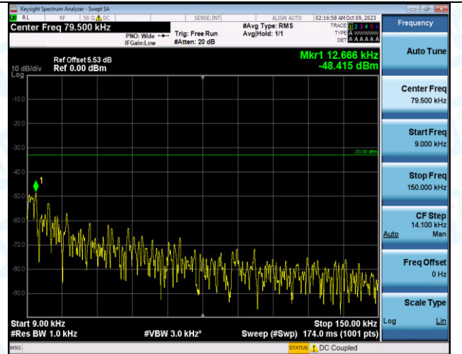
Band12_3MHz_16QAM_23165_15RB#0_0.009~0.15_0.00 9~0.15
