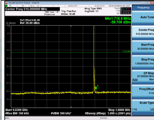
Band12_5MHz_QPSK_23035_1RB#0_30~1000_30~1000
