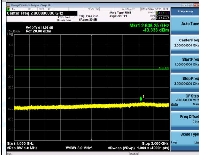
Band12_3MHz_16QAM_23095_1RB#0_1000~3000_1000 ~3000
