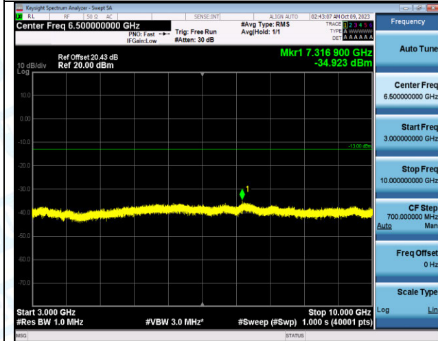
Band12_5MHz_QPSK_23035_25RB#0_3000~10000_3000~10000 0~10000
