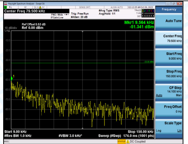
Band12_3MHz_16QAM_23095_1RB#0_0.009~0.15_0.009 ~0.15
