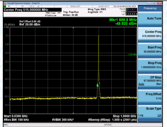
Band12_3MHz_16QAM_23095_15RB#0_30~1000_30~10
