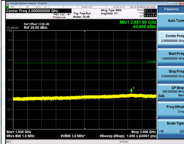
Band12_3MHz_16QAM_23095_15RB#0_1000~3000_1000~3000
