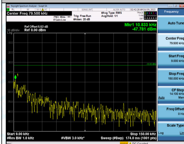
Band12_5MHz_QPSK_23035_25RB#0_0.009~0.15_0.009~0.15
