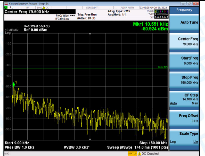
Band12_5MHz_16QAM_23035_25RB#0_0.009~0.15_0.009~0.15 9~0.15
