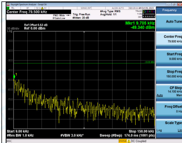
Band12_3MHz_QPSK_23095_15RB#0_0.009~0.15_0.00 9~0.15
