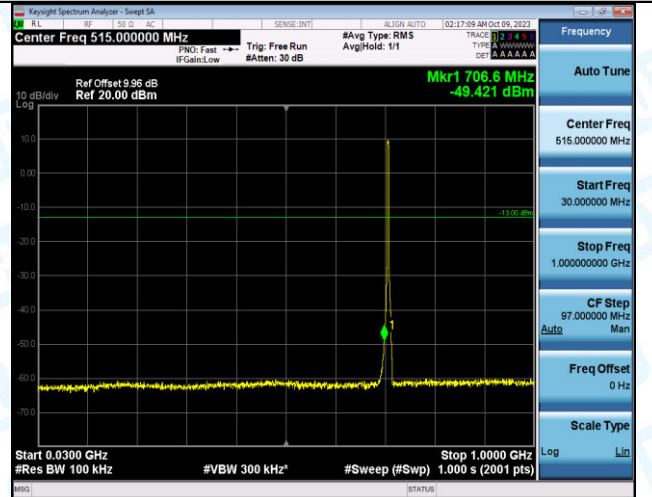
Band12_3MHz_16QAM_23165_15RB#0_30~1000_30~10 00
