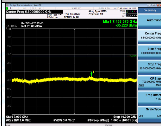
Band12_3MHz_QPSK_23095_15RB#0_3000~10000_300 0~10000
