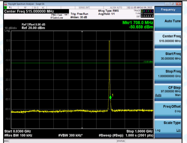
Band12_3MHz_16QAM_23025_15RB#0_30~1000_30~1000 00
