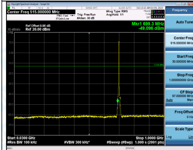
Band12_3MHz_QPSK_23095_15RB#0_30~1000_30~100 0
