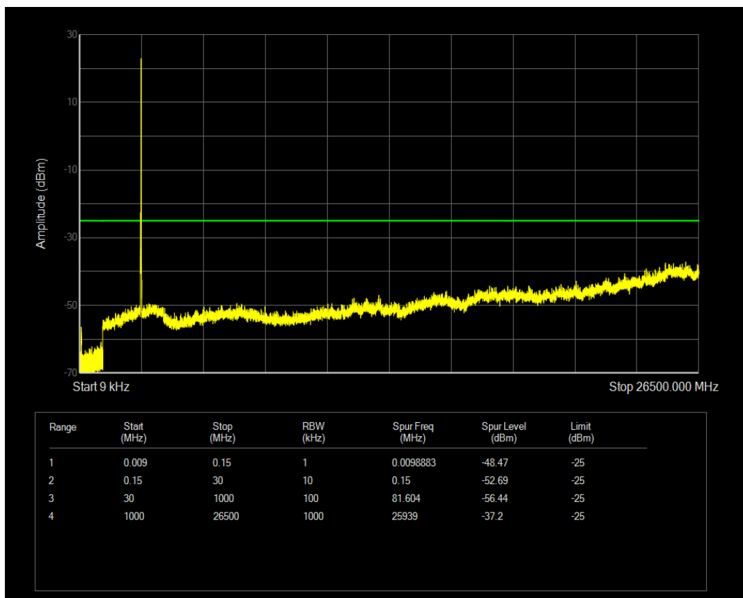
Band41 QPSK BW=10MHz Channel=40390 RB Size=1 Position=#0
