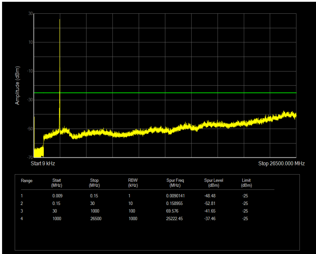
Band41 16QAM BW=15MHz Channel=41065 RB Size=75 Position=#0
