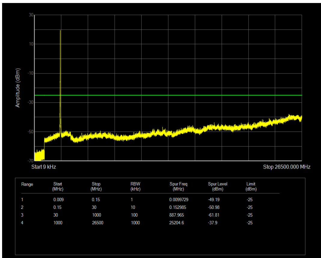
Band41 16QAM BW=15MHz Channel=40415 RB Size=1 Position=#0
