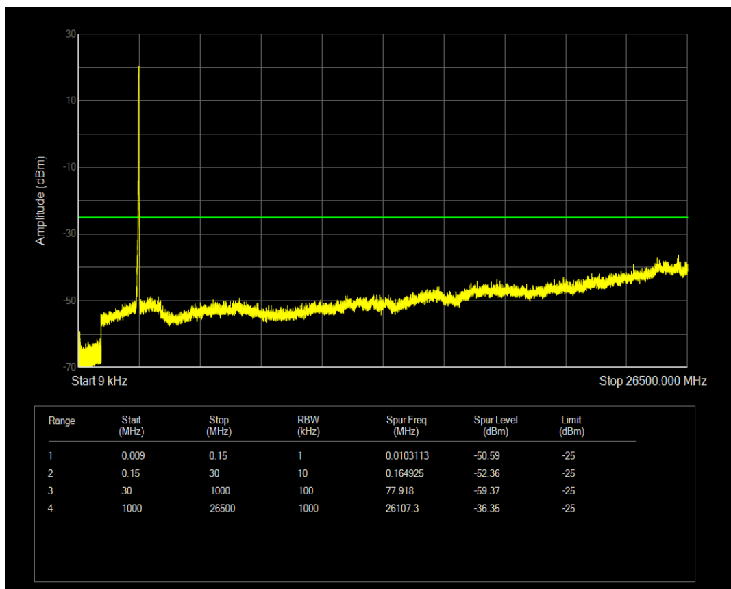
Band41 16QAM BW=20MHz Channel=41040 RB Size=1 Position=#0
