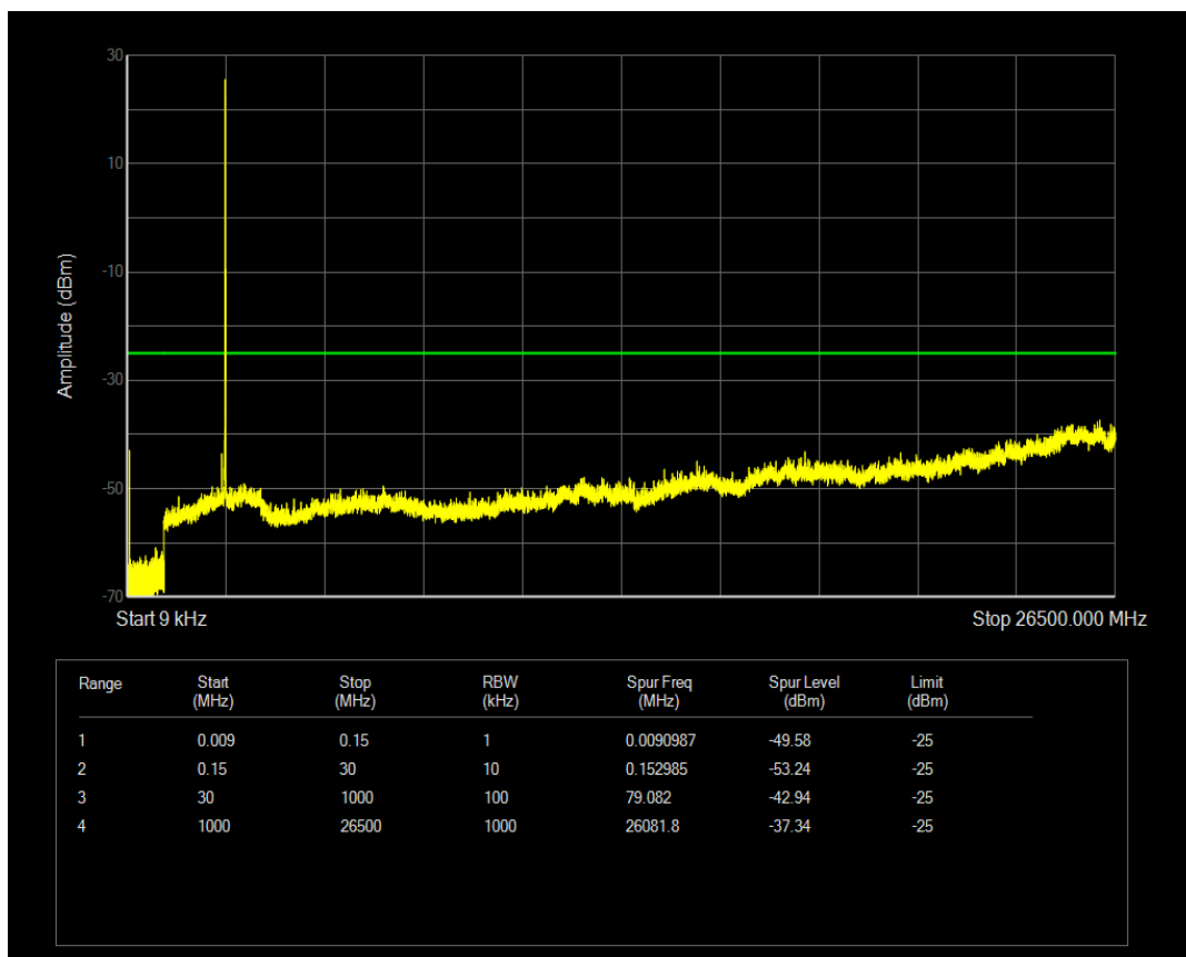
Band41 QPSK BW=5MHz Channel=41115 RB Size=25 Position=#0
