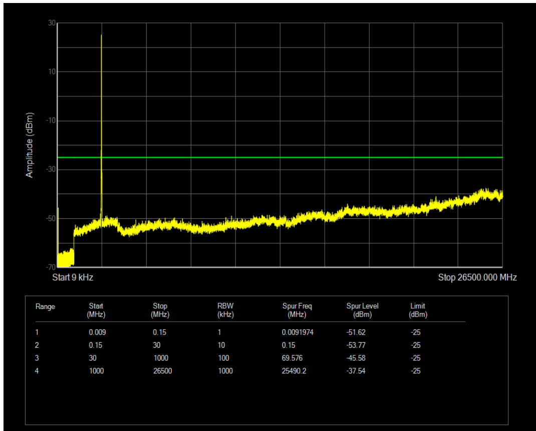
Band41 QPSK BW=15MHz Channel=41065 RB Size=75 Position=#0
