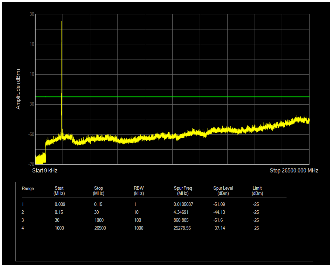
Band41 16QAM BW=10MHz Channel=40390 RB Size=1 Position=#0
