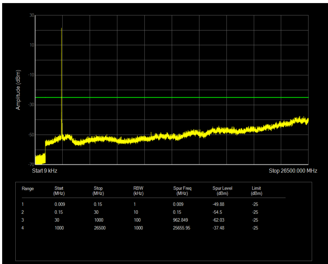
Band41 QPSK BW=5MHz Channel=40740 RB Size=1 Position=#0
