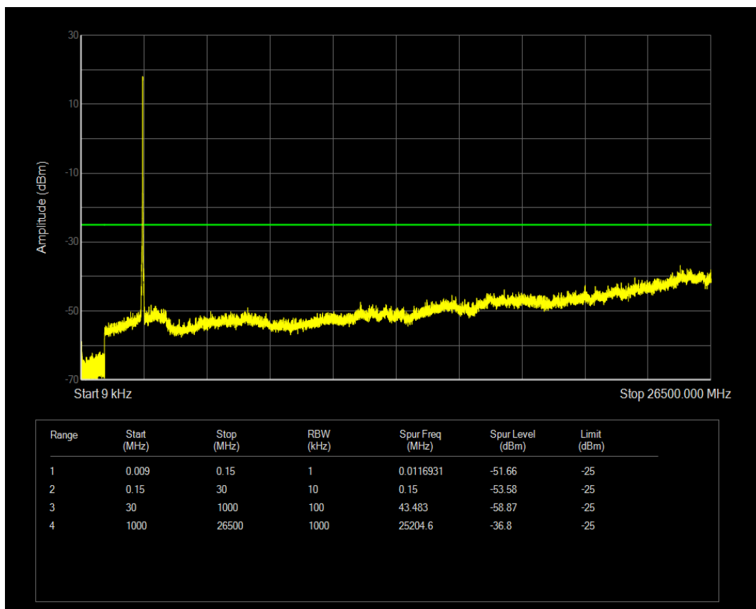
Band41 QPSK BW=15MHz Channel=41065 RB Size=1 Position=#0
