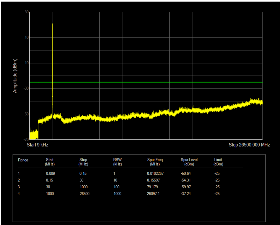
Band41 QPSK BW=15MHz Channel=40415 RB Size=1 Position=#0
