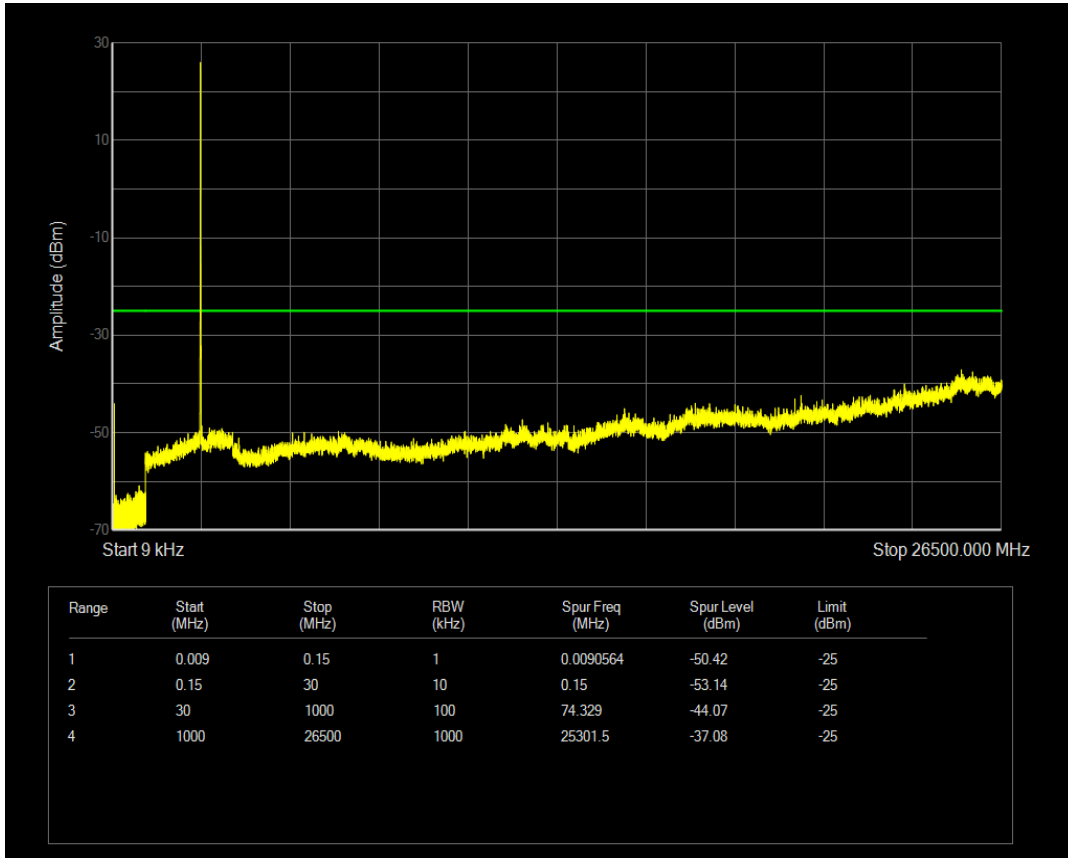
Band41 16QAM BW=10MHz Channel=41090 RB Size=50 Position=#0
