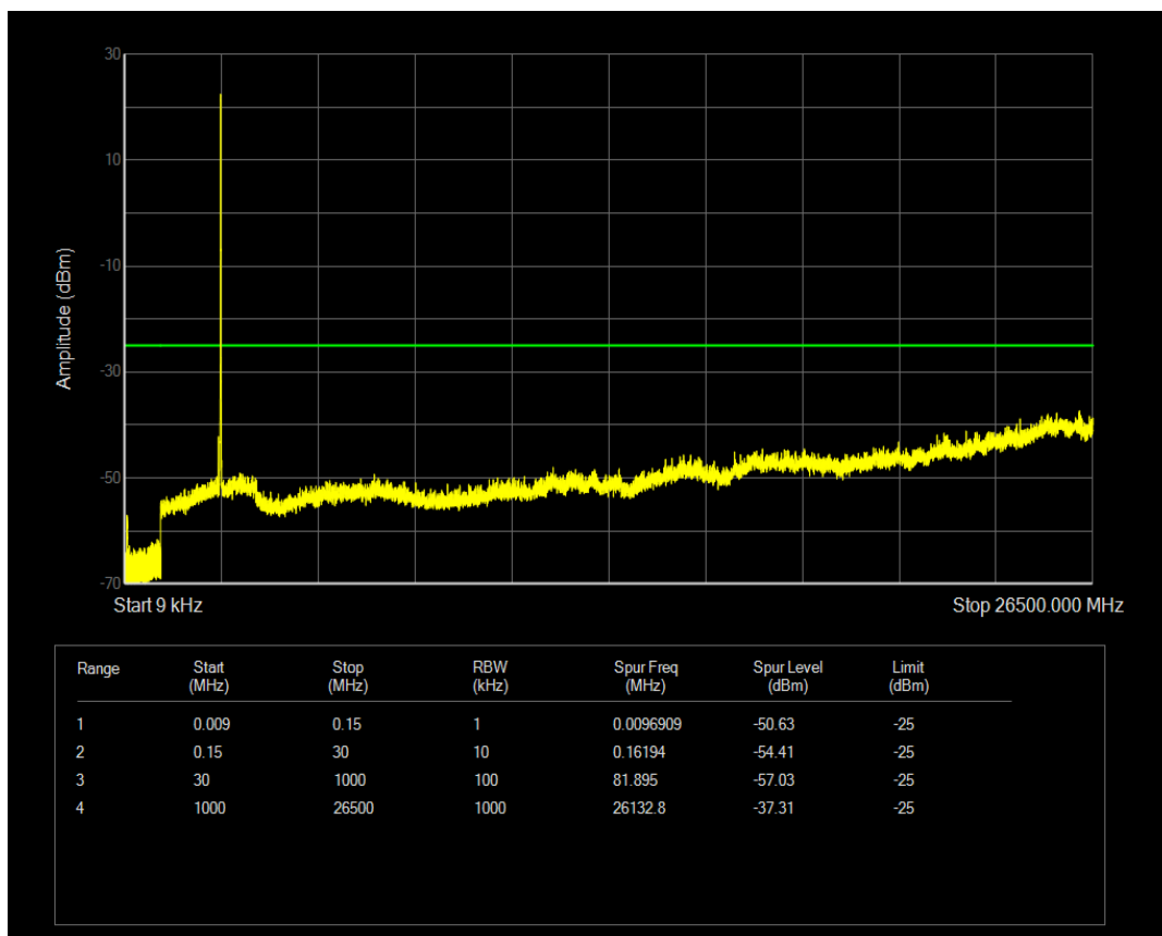
Band41 16QAM BW=5MHz Channel=41115 RB Size=1 Position=#0
