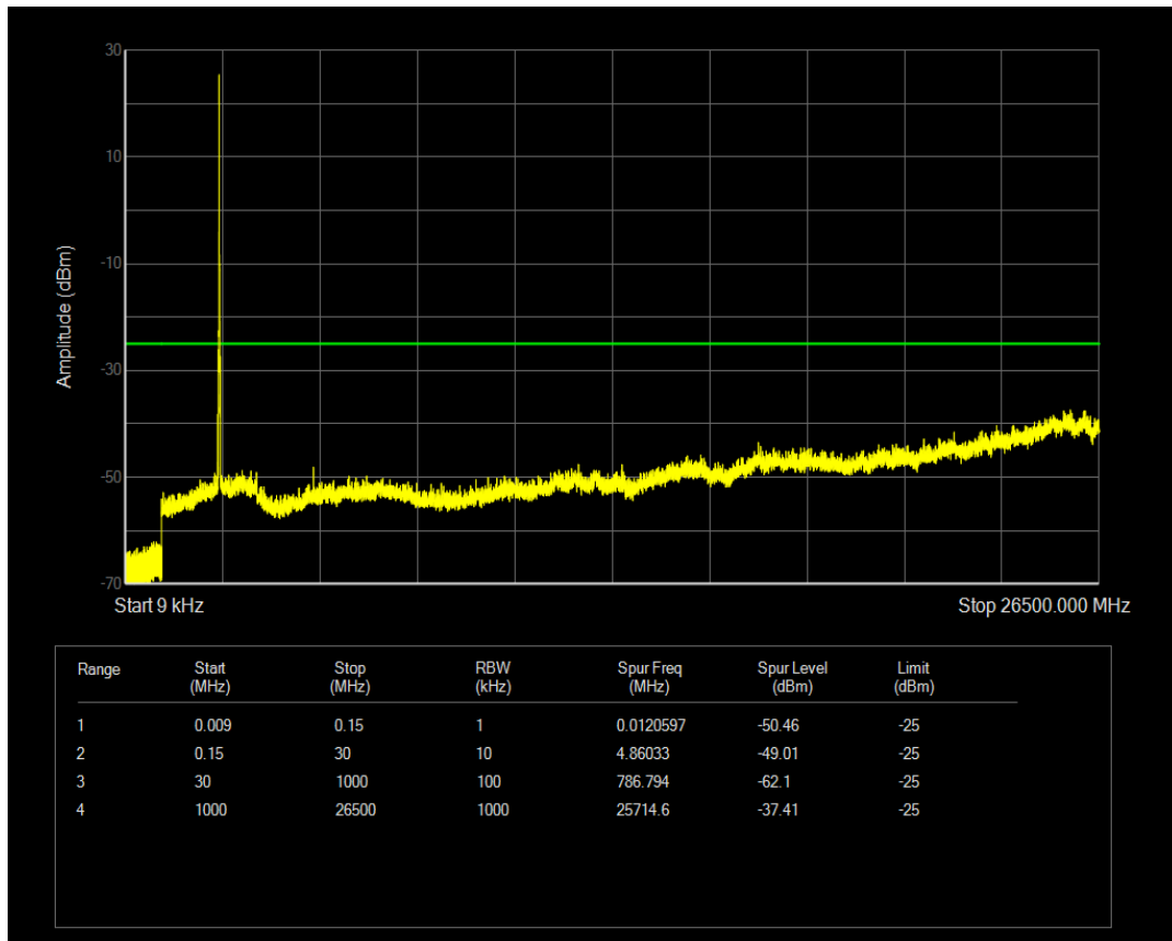
Band41 QPSK BW=20MHz Channel=40440 RB Size=100 Position=#0
