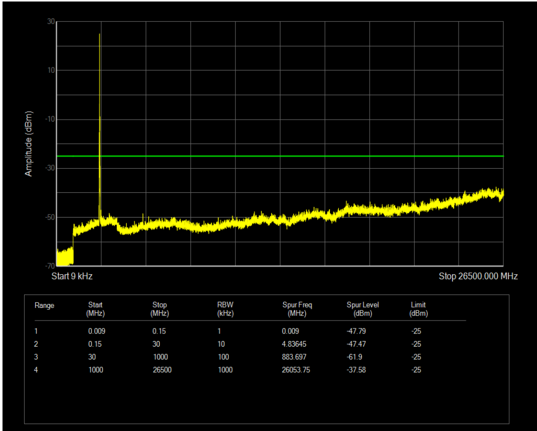
Band41 16QAM BW=20MHz Channel=40440 RB Size=100 Position=#0
