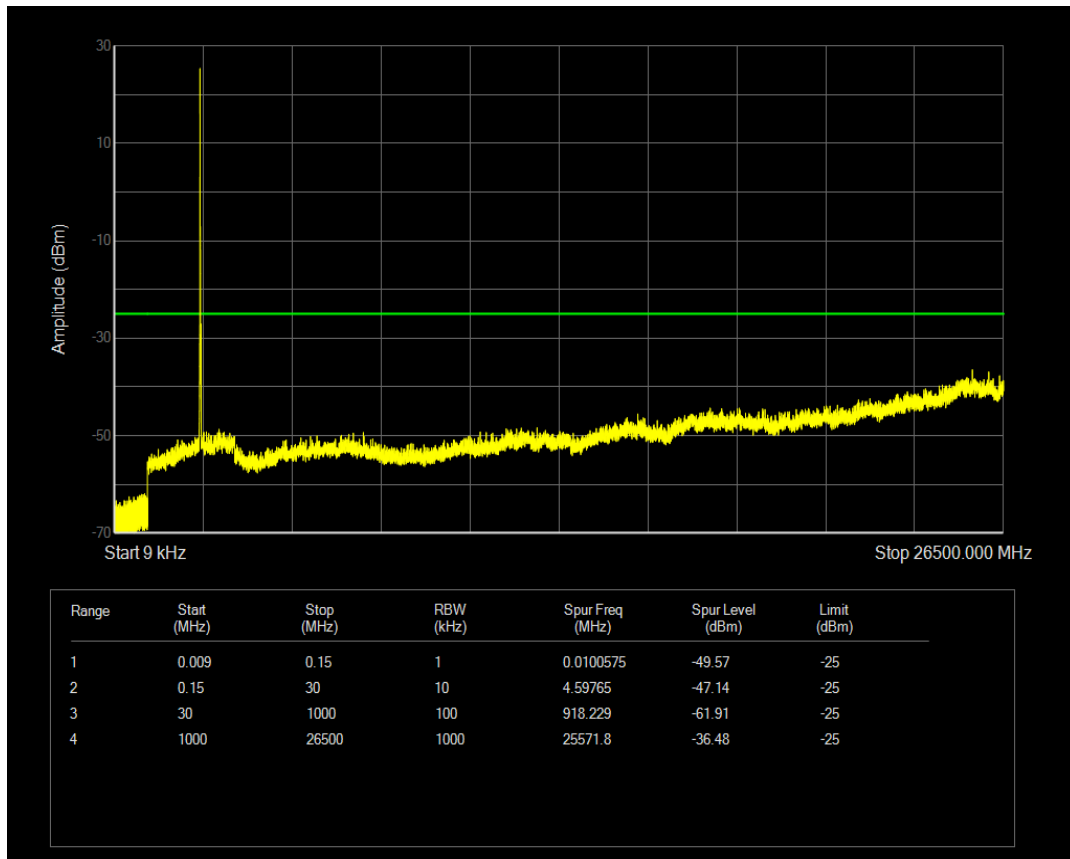
Band41 16QAM BW=15MHz Channel=40415 RB Size=75 Position=#0
