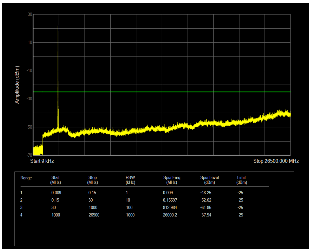
Band41 16QAM BW=5MHz Channel=40365 RB Size=1 Position=#0
