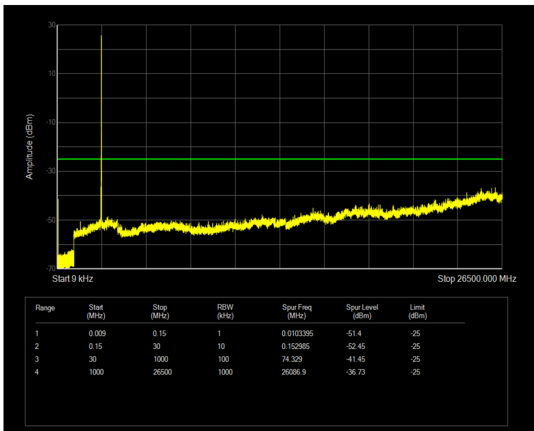
Band41 QPSK BW=10MHz Channel=41090 RB Size=50 Position=#0
