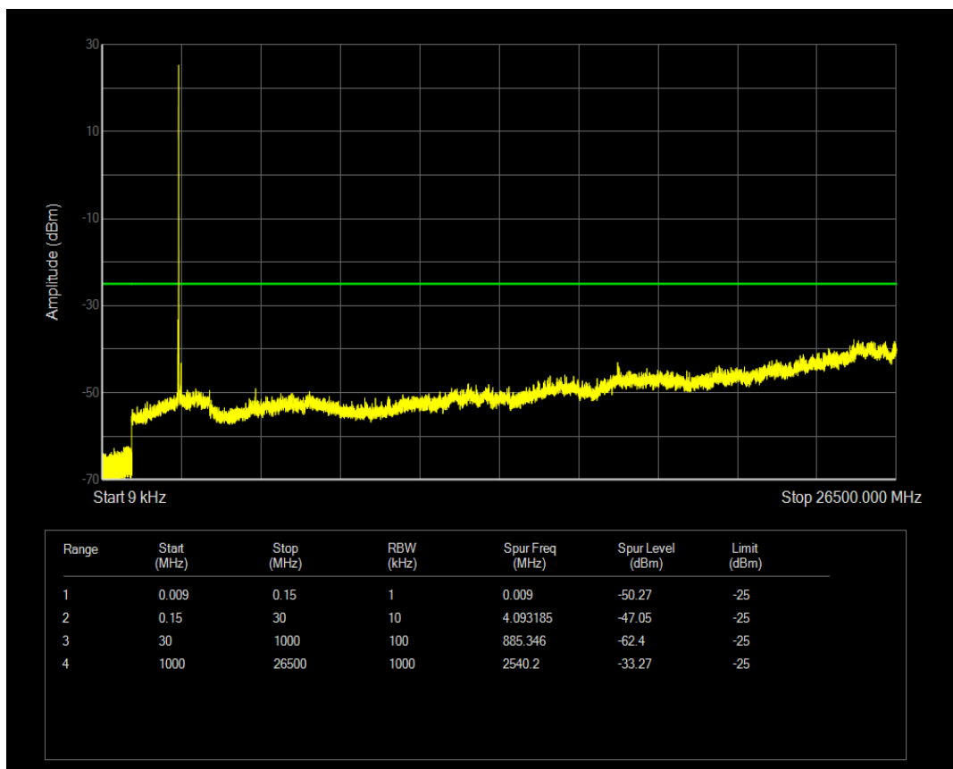
Band41 16QAM BW=5MHz Channel=40365 RB Size=25 Position=#0
