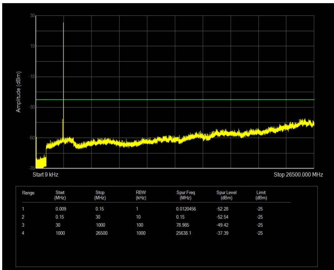
Band41 16QAM BW=5MHz Channel=41115 RB Size=25 Position=#0
