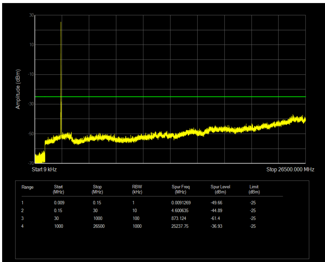
Band41 QPSK BW=15MHz Channel=40415 RB Size=75 Position=#0
