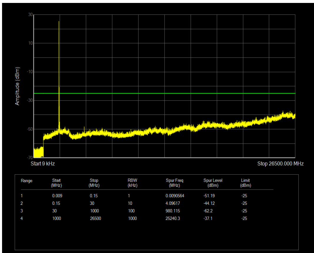
Band41 QPSK BW=5MHz Channel=40365 RB Size=25 Position=#0
