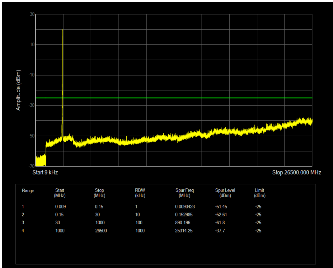
Band41 16QAM BW=10MHz Channel=40390 RB Size=50 Position=#0
