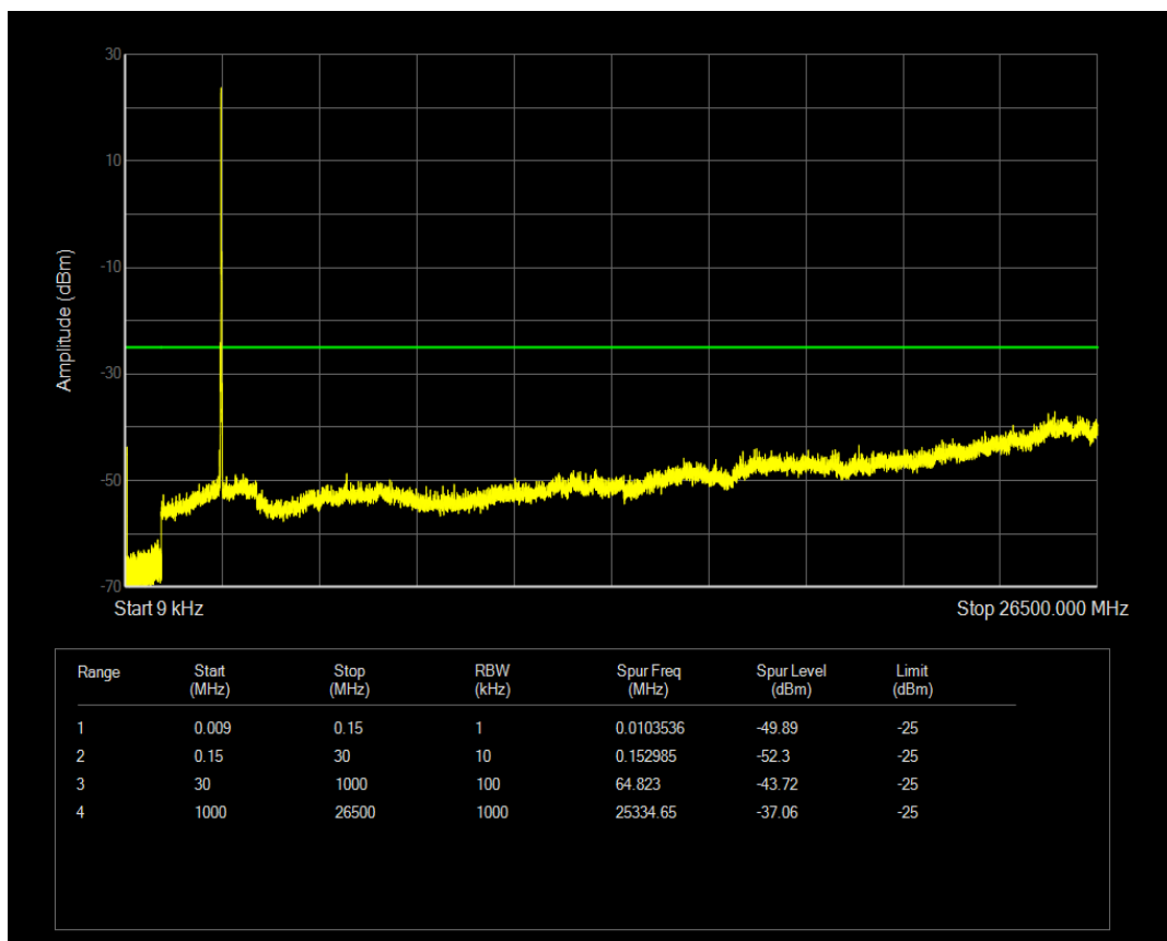
Band41 QPSK BW=20MHz Channel=41040 RB Size=100 Position=#0
