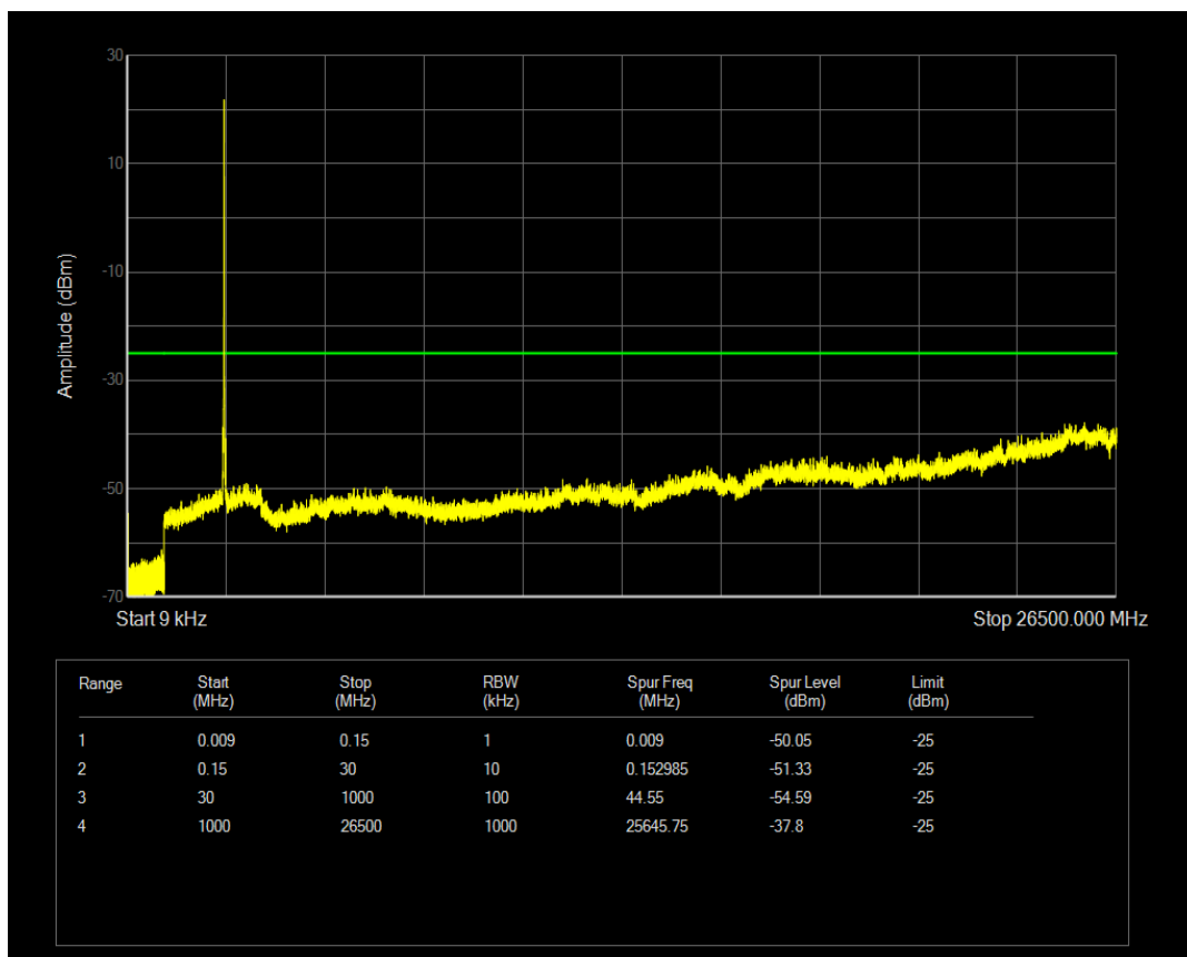
Band41 QPSK BW=5MHz Channel=41115 RB Size=1 Position=#0
