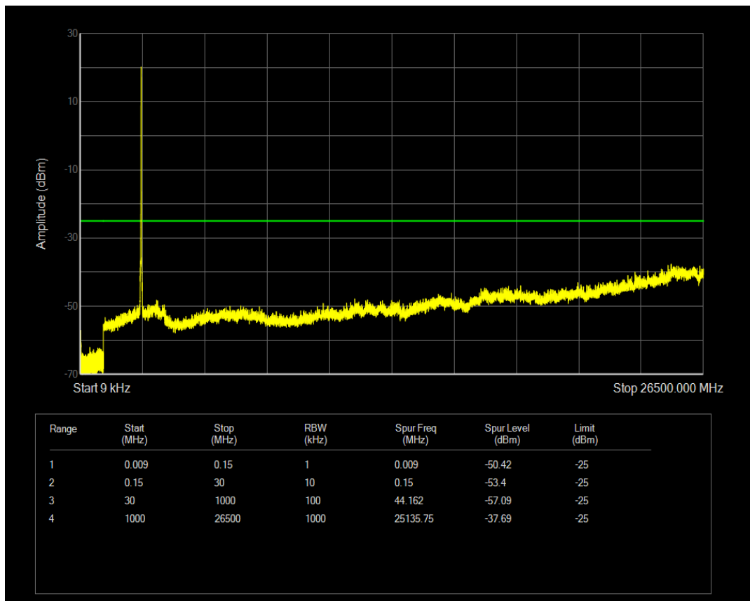
Band41 QPSK BW=10MHz Channel=41090 RB Size=1 Position=#0
