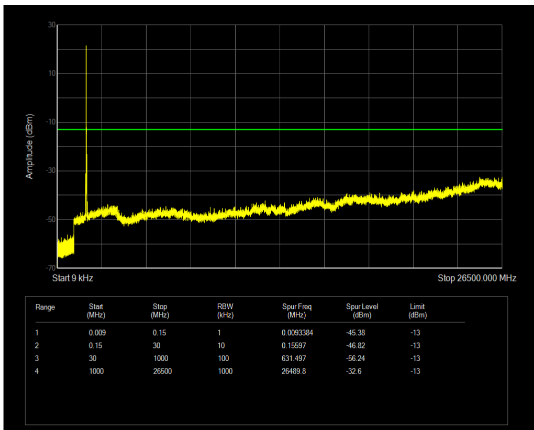
Band41 QPSK BW=5MHz Channel=40365 RB Size=1 Position=#0
