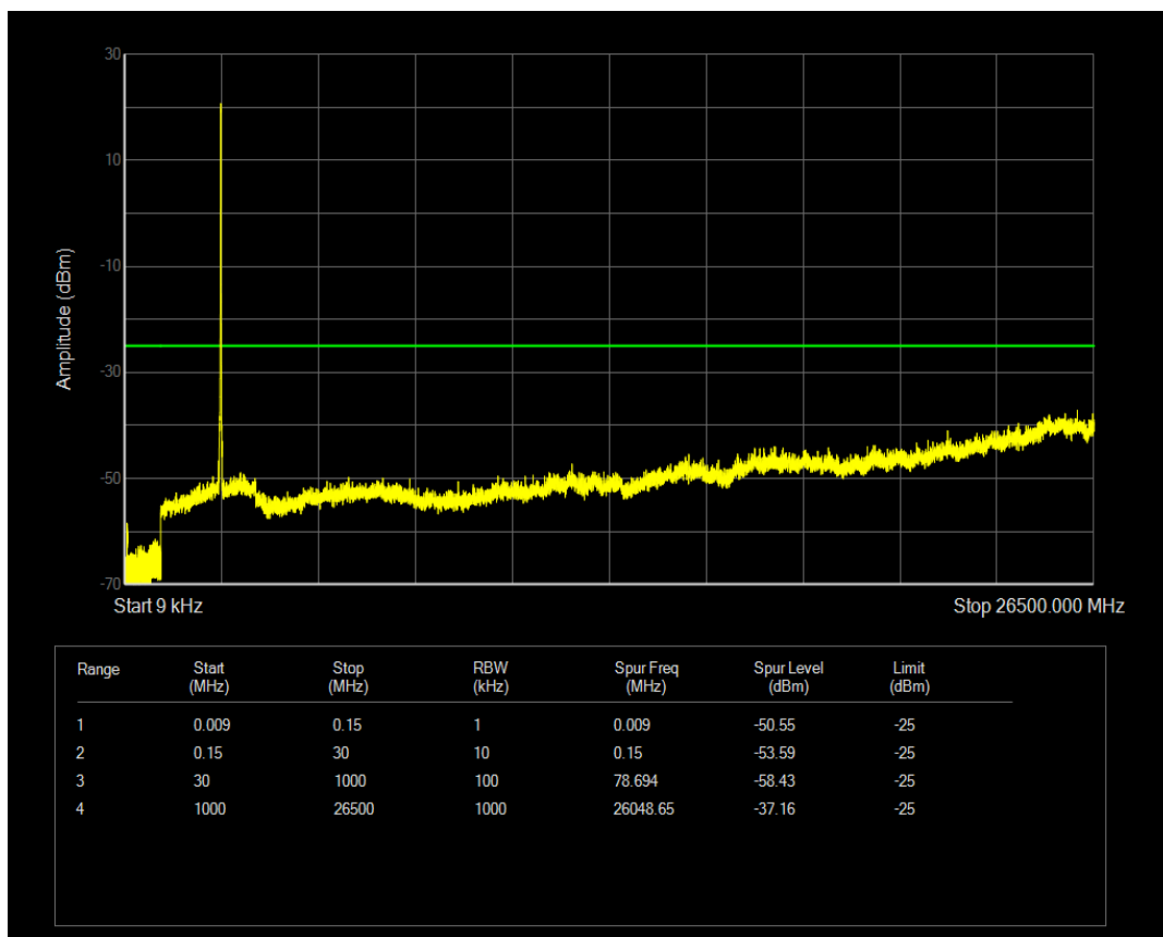
Band41 16QAM BW=10MHz Channel=41090 RB Size=1 Position=#0
