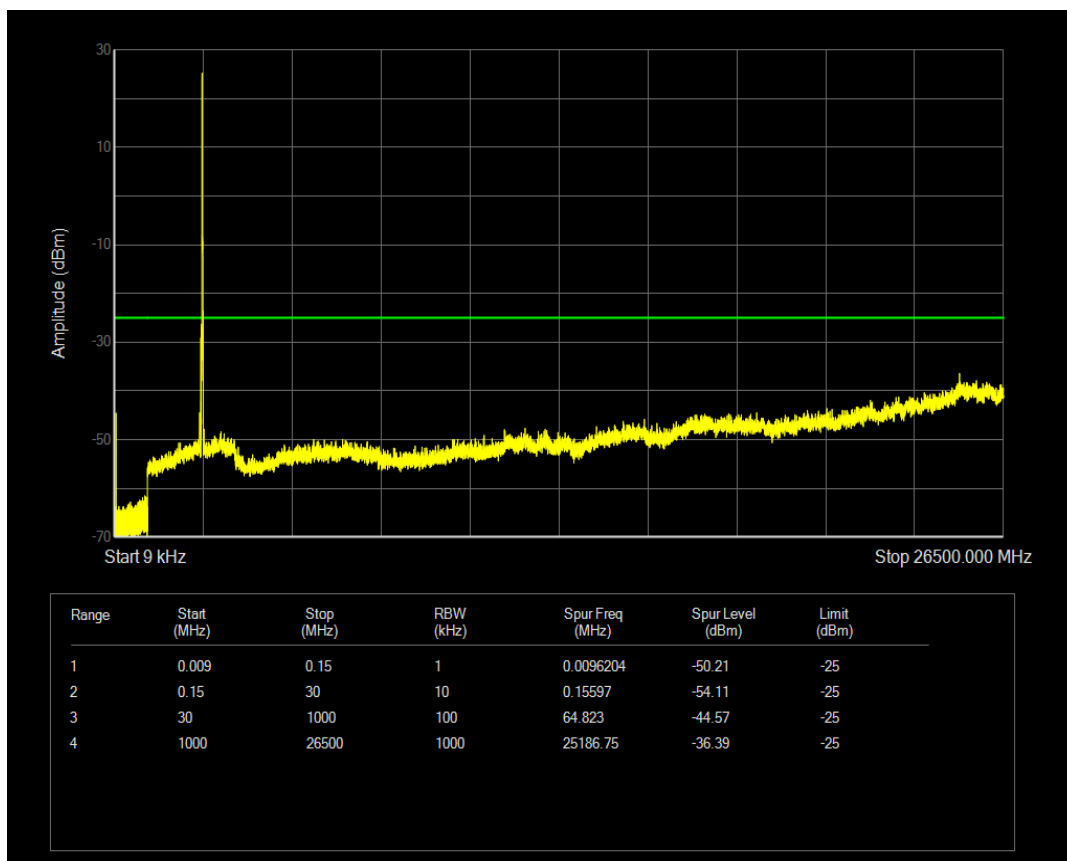
Band41 16QAM BW=20MHz Channel=41040 RB Size=100 Position=#0
