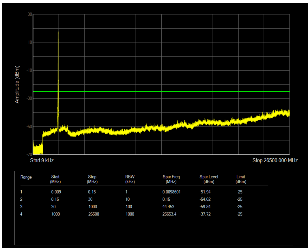
Band41 QPSK BW=20MHz Channel=41040 RB Size=1 Position=#0
