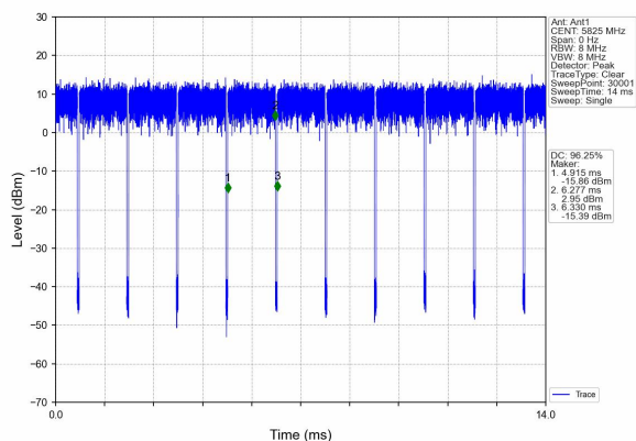
(802.11a) channel 165
