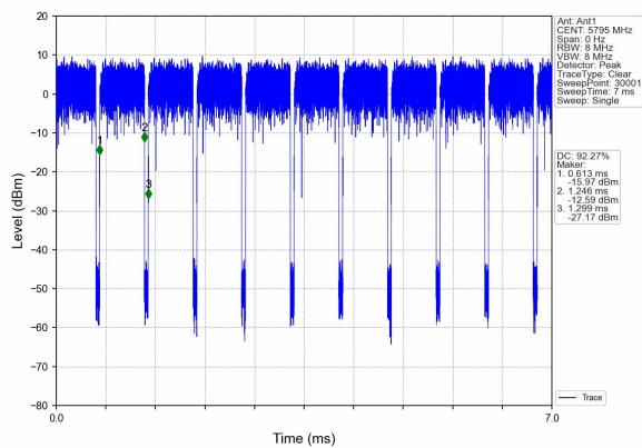
(802.11 ac40) channel 159
