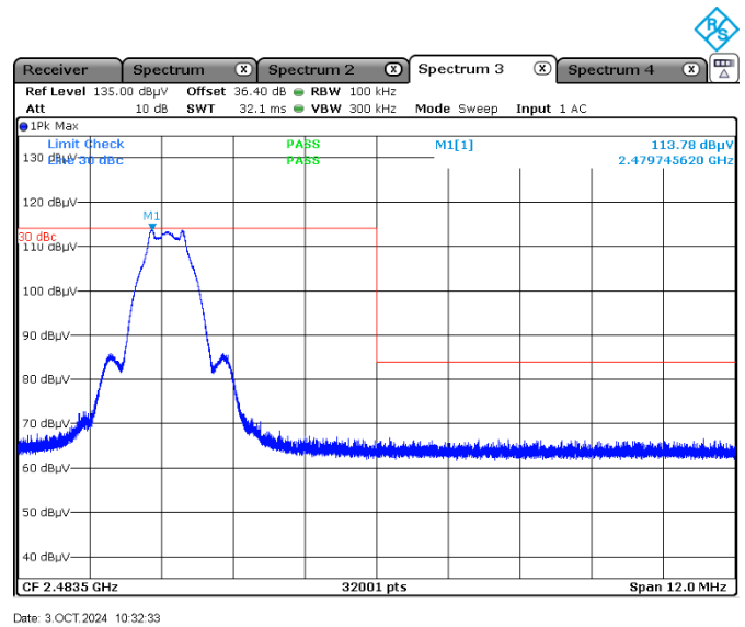
Figure 7.7-11: Band edge spurious emissions at 2483.5 MHz, non-restricted band edge, high channel
