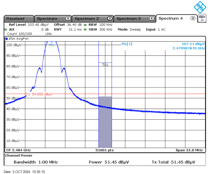
Figure 7.7-15: Band edge spurious emissions at 2483.5 MHz Average, restricted bands, high channel
