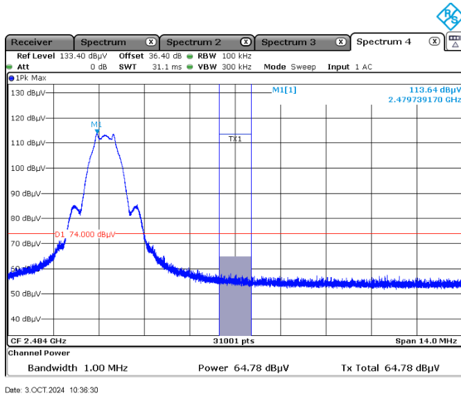
Figure 7.7-14: Band edge spurious emissions at 2483.5 MHz Peak, restricted bands, high channel
