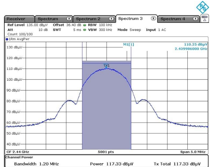
Figure 7.6-2: Output power on mid channel
