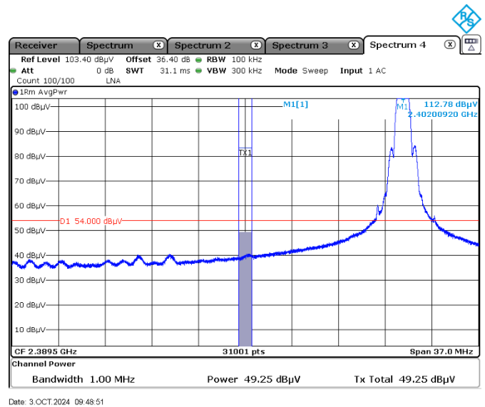
Figure 7.7-13: Band edge spurious emissions at 2390 MHz Average, restricted bands, low channel
