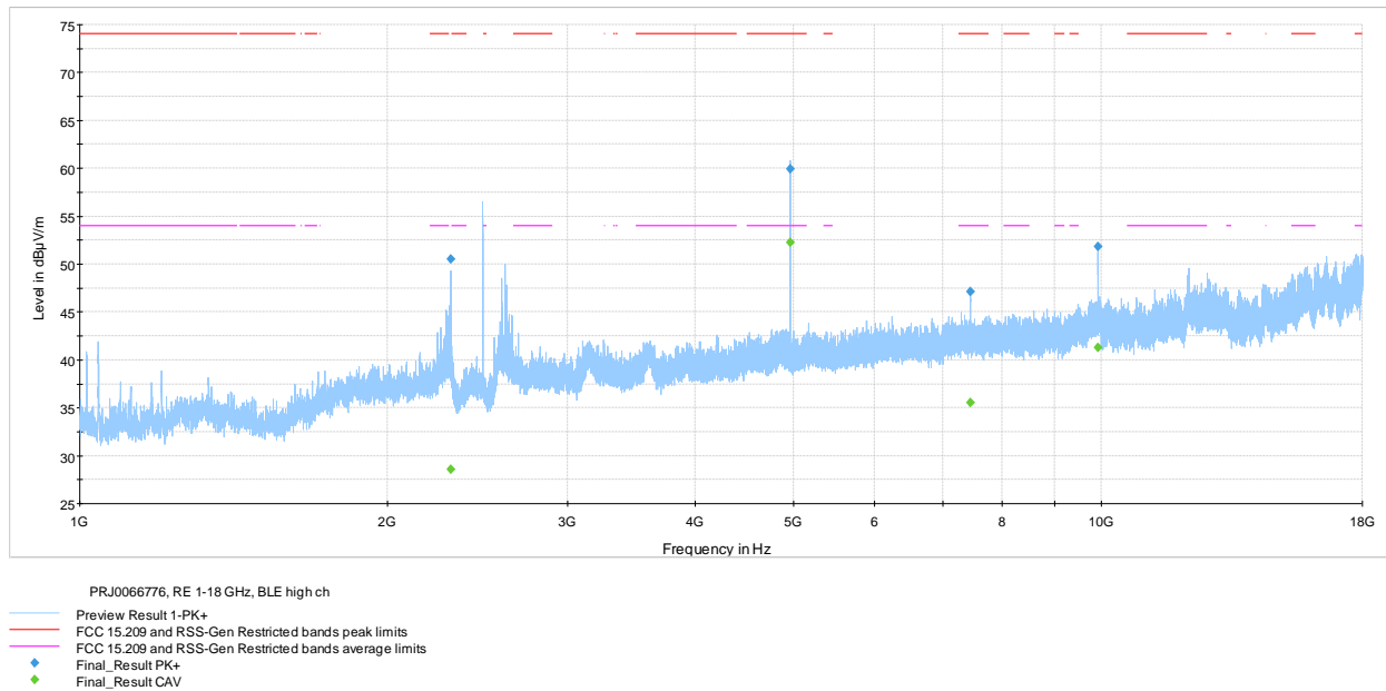
Figure 7.7-6: Radiated spurious emissions 1-18 GHz high channel
