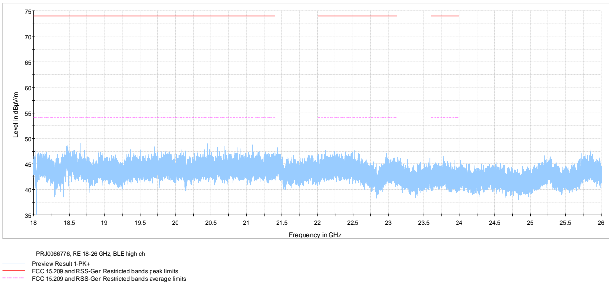
Figure 7.7-9: Radiated spurious emissions 18-26 GHz high channel
