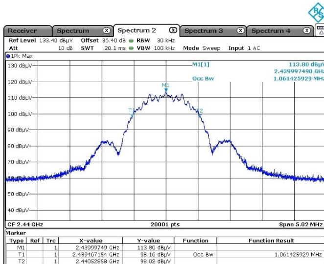
Figure 7.5-5: 99% occupied bandwidth on mid channel
