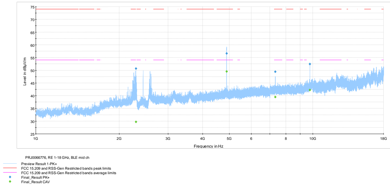
Figure 7.7-5: Radiated spurious emissions 1-18 GHz mid channel
