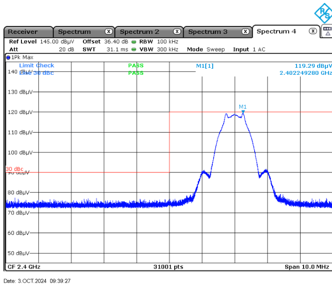
Figure 7.7-10: Band edge spurious emissions at 2400 MHz, non-restricted band edge, low channel
