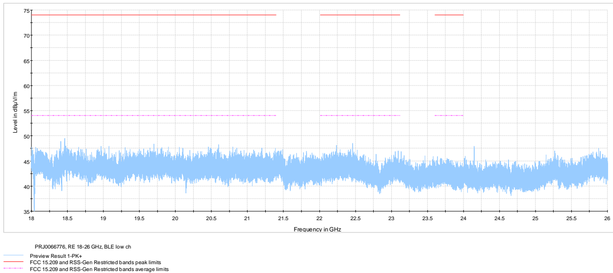
Figure 7.7-7: Radiated spurious emissions 18-26 GHz low channel
