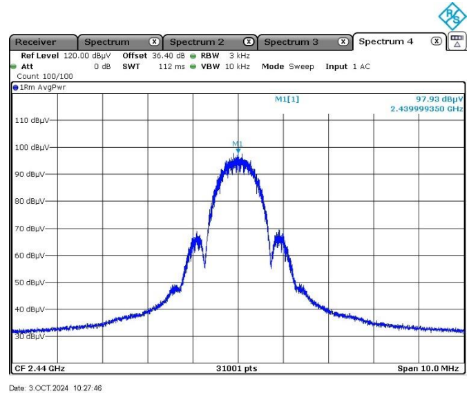
Figure 7.8-2: PSD on mid channel
