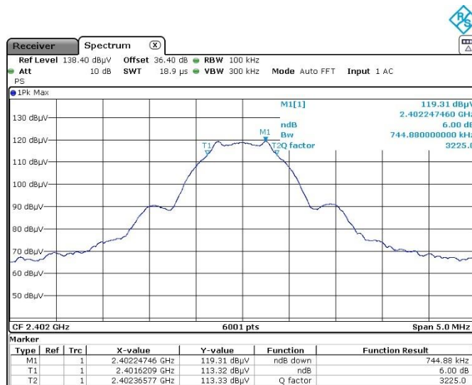
Figure 7.5-1: 6 dB bandwidth on low channel
