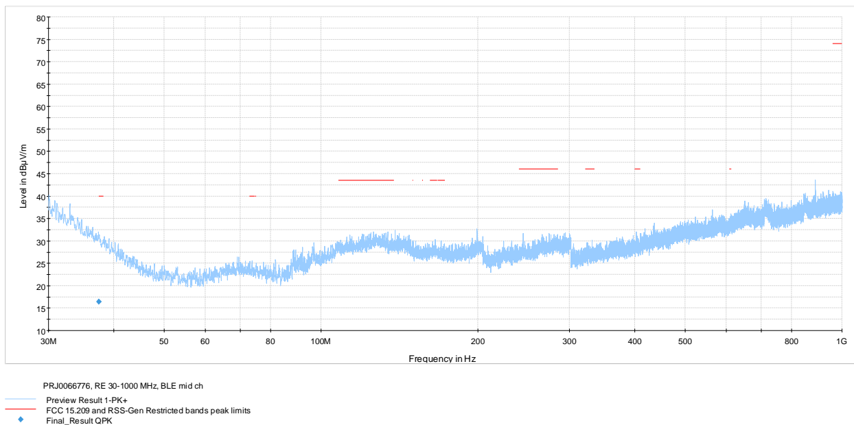
Figure 7.7-2: Radiated spurious emissions 30-1000 MHz mid channel
