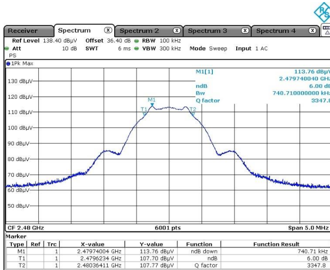
Figure 7.5-3: 6 dB bandwidth on high channel
