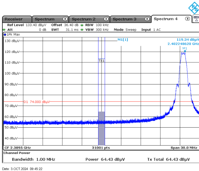
Figure 7.7-12: Band edge spurious emissions at 2390 MHz Peak, restricted bands, low channel
