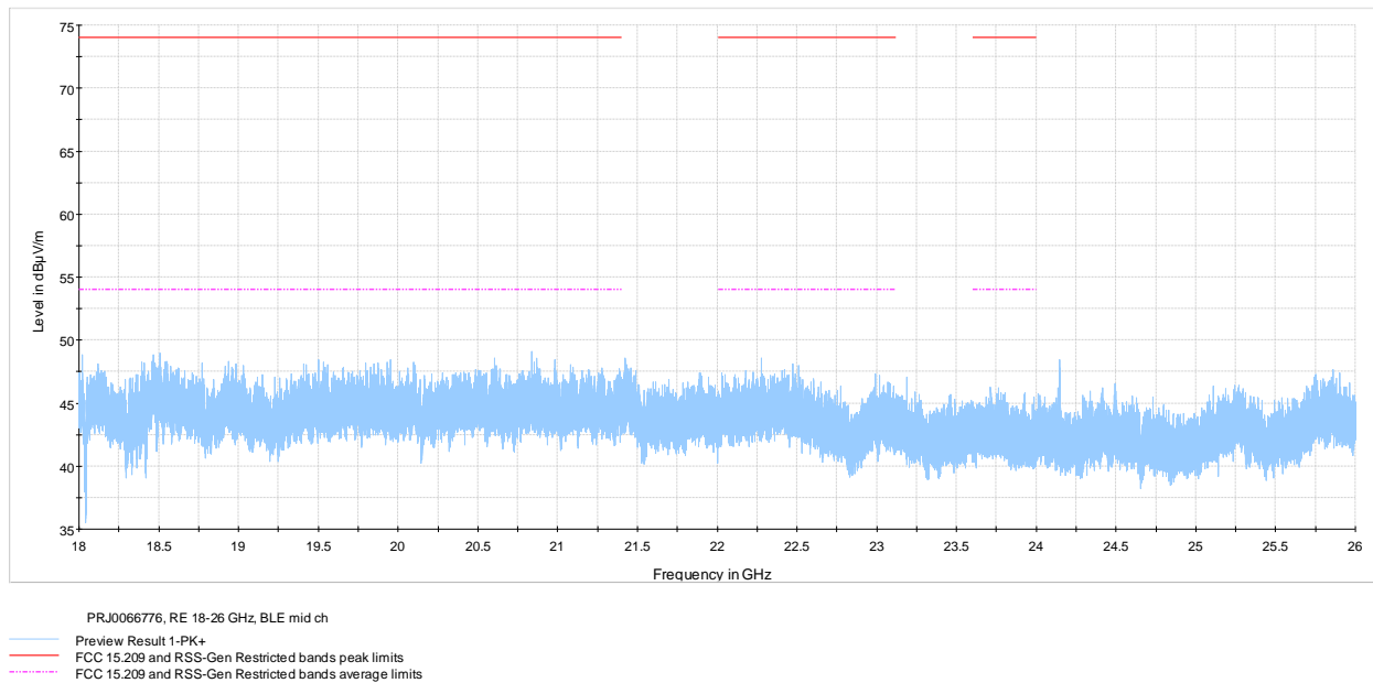
Figure 7.7-8: Radiated spurious emissions 18-26 GHz mid channel
