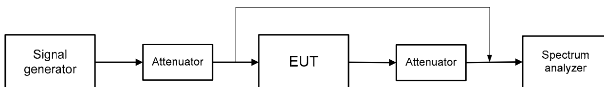
Figure 7.1.1 AGC Threshold level test setup
