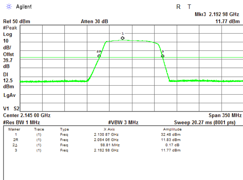
Plot 7.4.1 Out-of-band rejection test result
