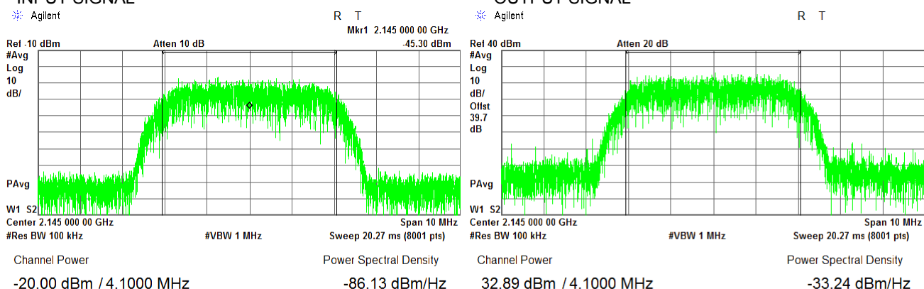
Plot 7.1.2 RF output power measurements at mid frequency carrier
