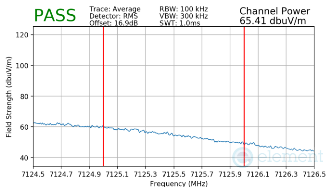
Plot 7-698. Antenna 1b Radiated Upper Band Edge (Average – UNII Band 8)
