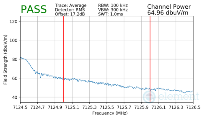
Plot 7-702. Antenna 1b Radiated Upper Band Edge (Average – UNII Band 8)
