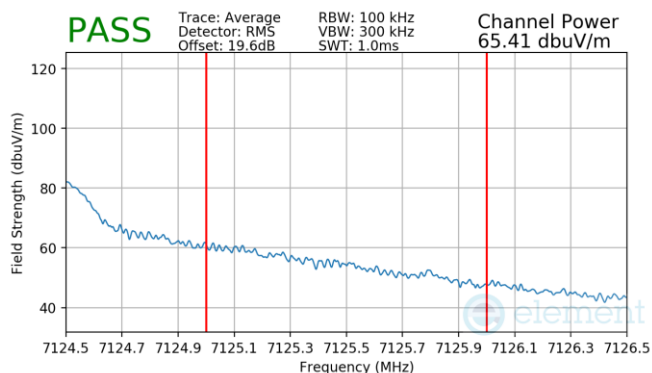
Plot 7-722. SDM Diversity Radiated Upper Band Edge (Average – UNII Band 8)
