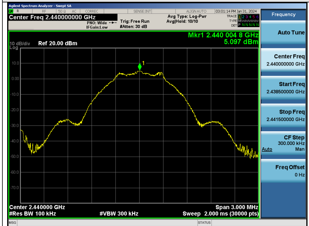
Test_Graph_LE2M_ANT1_2440_1Mbps_Reference Level
