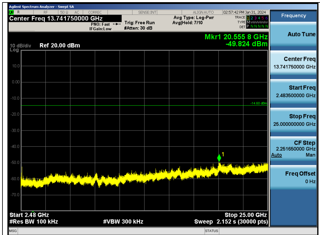
Test_Graph_LE2M_ANT1_2402_1Mbps_Higher Band Emissions
