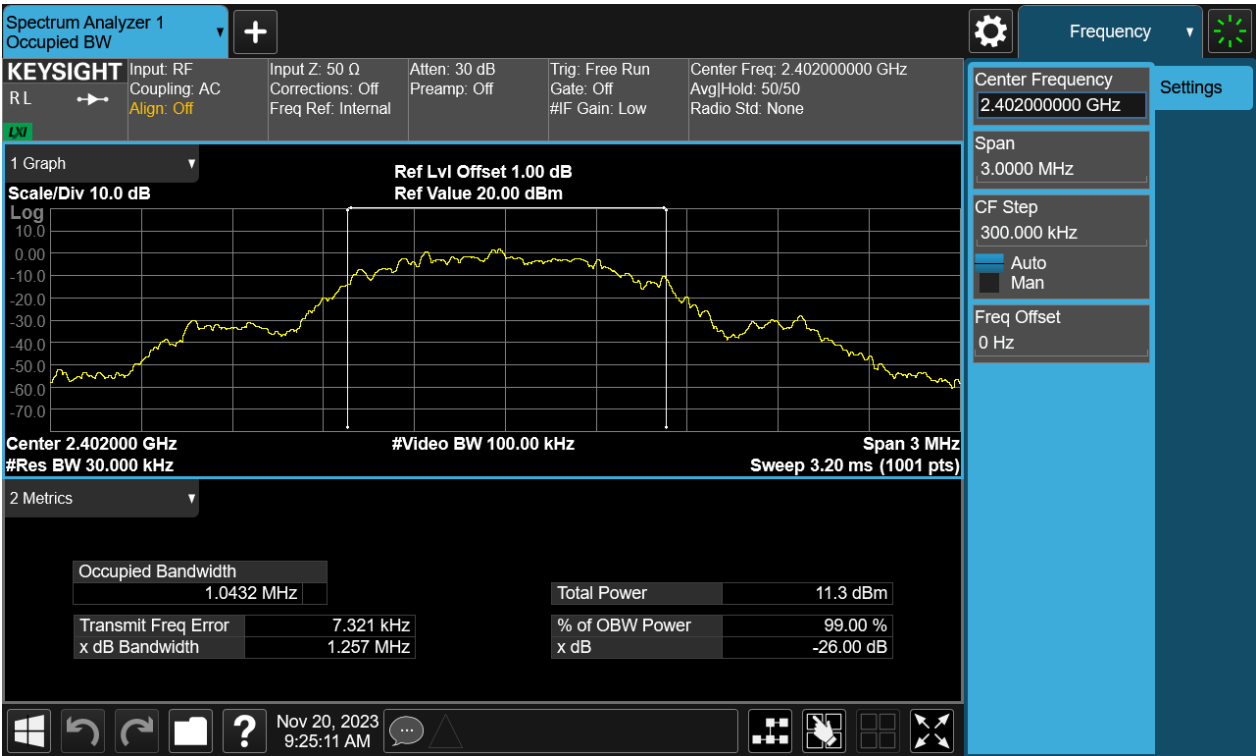
99% Bandwidth, 2402MHz
