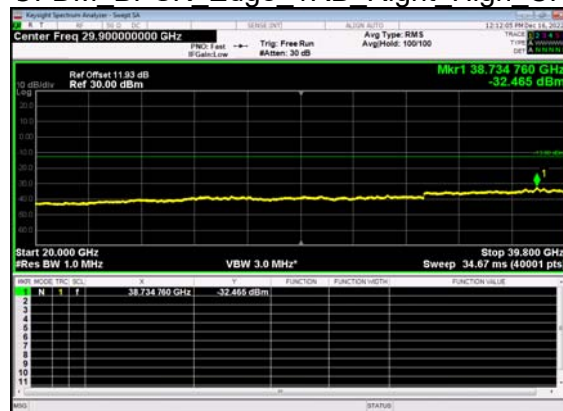
N77(100M)_DFT-s-OFDM BPSK Edge 1RB Right High CH
