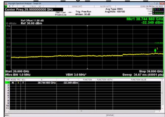
N77(100M)_DFT-s- OFDM BPSK Edge 1RB Left Mid CH
