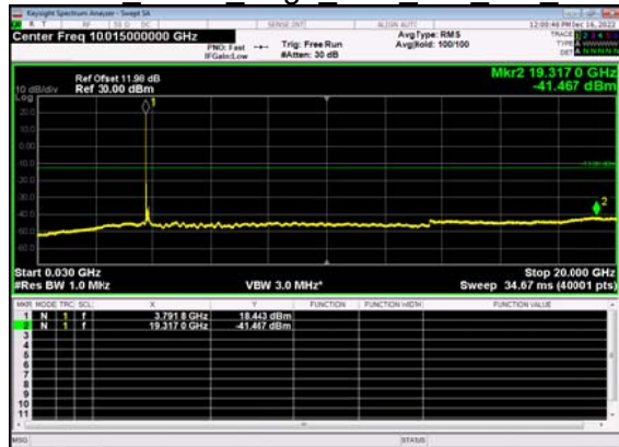
N77(100M)_DFT-s- OFDM BPSK Edge 1RB Left Mid CH
