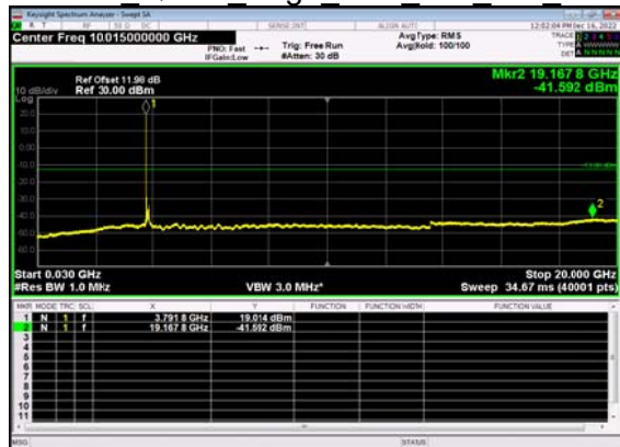
N77(100M)_DFT-s- OFDM QPSK Edge 1RB Left Mid CH
