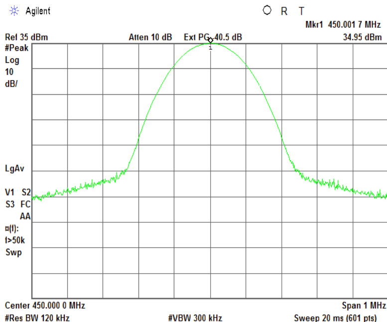
Plot 7.1.1 Peak output power test results at low frequency
