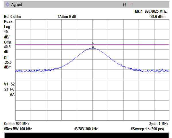
Plot 7.5.11 Spurious emission measurements in 600 - 1000 MHz range at mid carrier frequency
