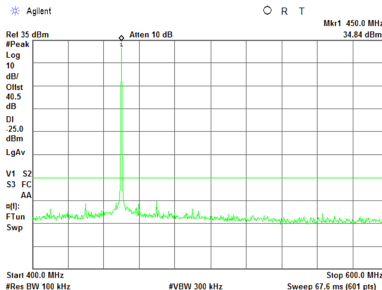
Plot 7.5.4 Spurious emission measurements in 400 - 600 MHz range at low carrier frequency
