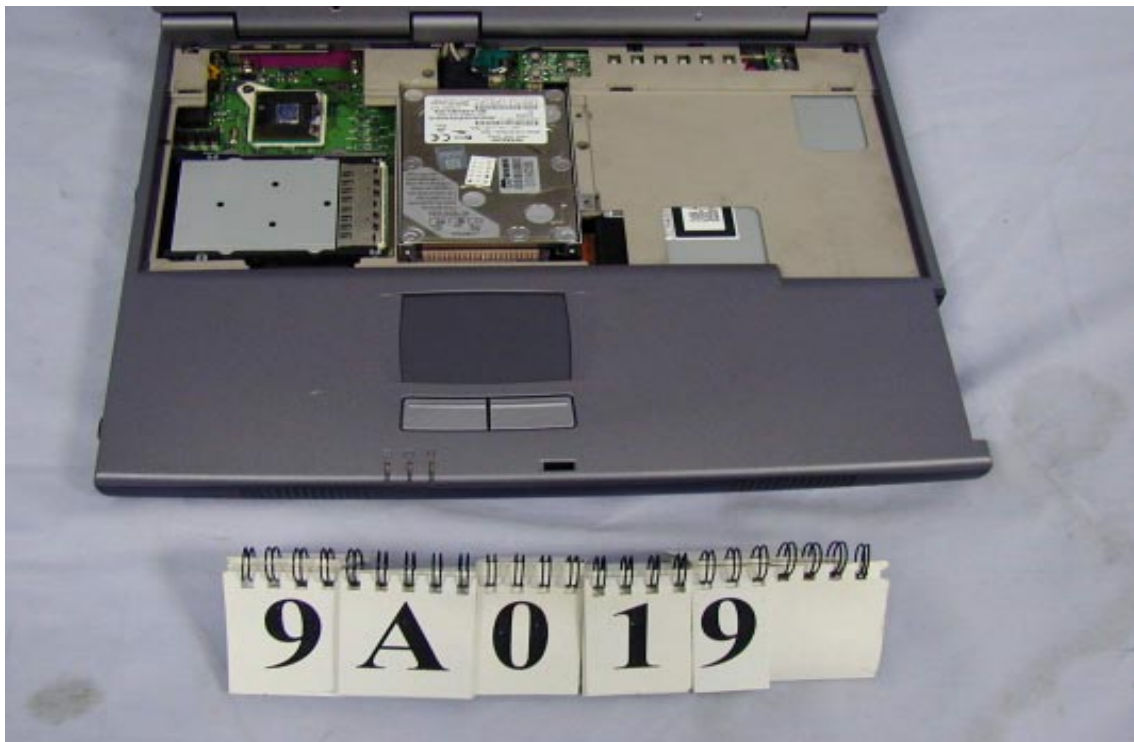
EUT Inside View 2
