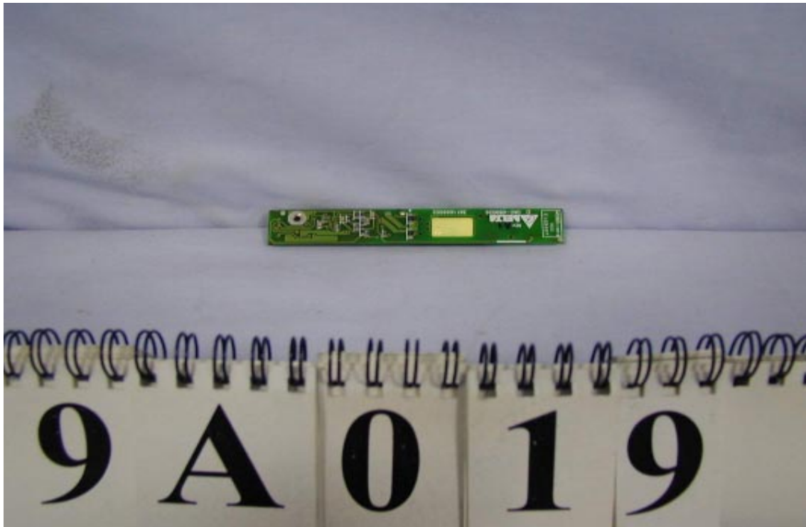
Convertor Solder Side View
