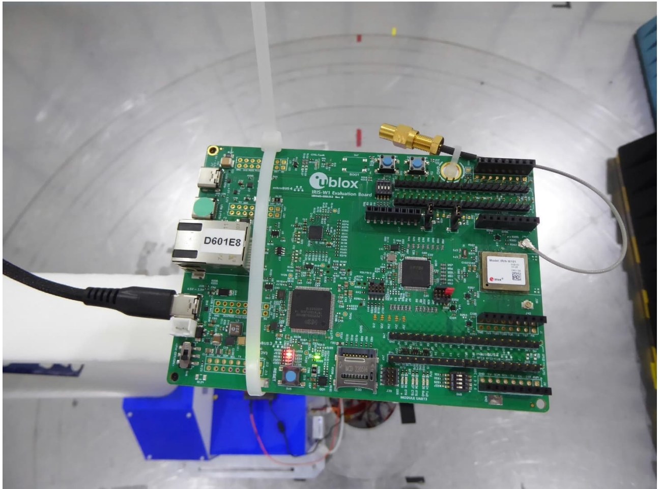
EUT on positioner
