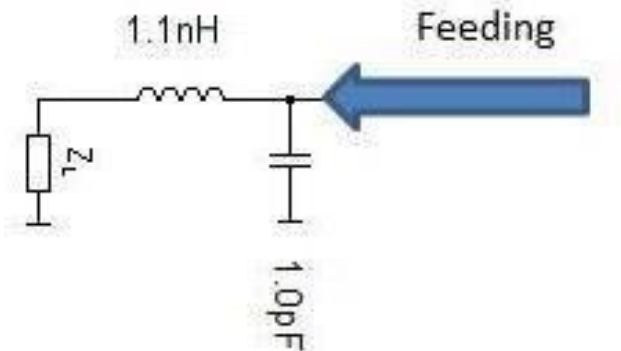
Suggested Matching Circuit
