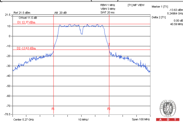
WHDI (40MHz)
