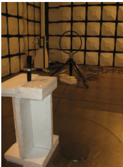
Photograph 1: Set-up for Radiation Measurement below 1GHz
