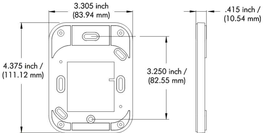
FIGURE 1. Model SWH-5100 Reader Backplate (includes tamper switch magnet)
