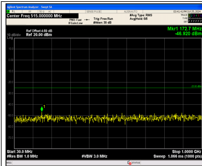
Band7-5MHz-16QAM-21100-1RB#0-Range1:30~100 0MHz
