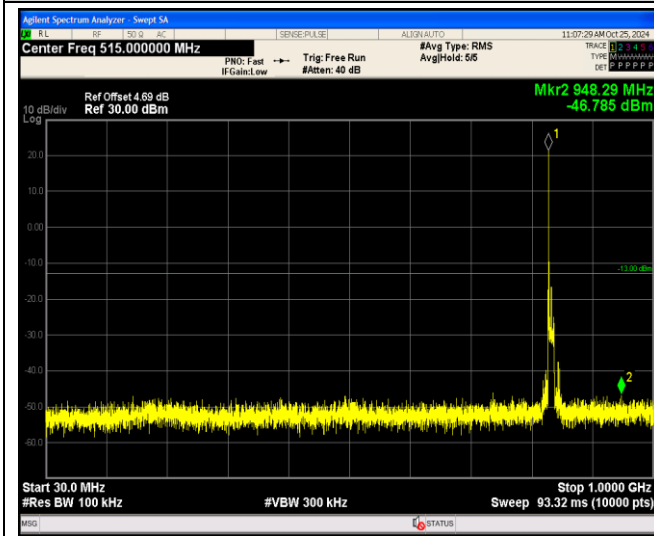
Band5-10MHz-16QAM-20525-1RB#0-Range1:30~1000MHz
