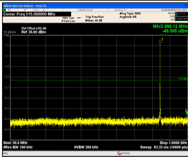
Band5-1.4MHz-64QAM-20643-1RB#0-Range1:30~1000MHz
