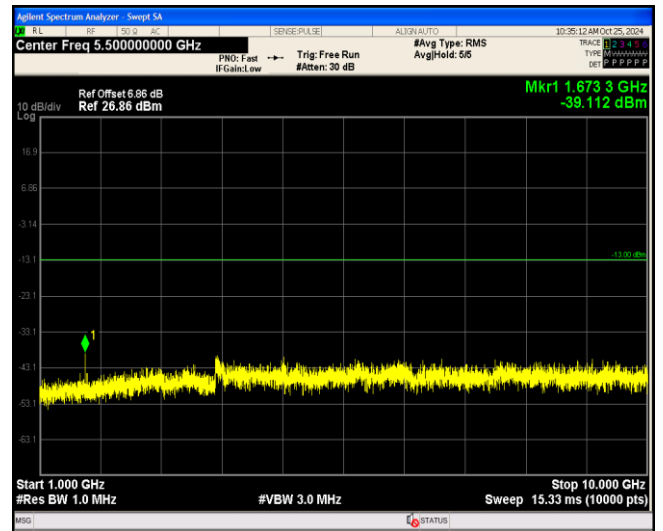
Band5-1.4MHz-64QAM-20643-1RB#0-Range2:1000~10000MHz
