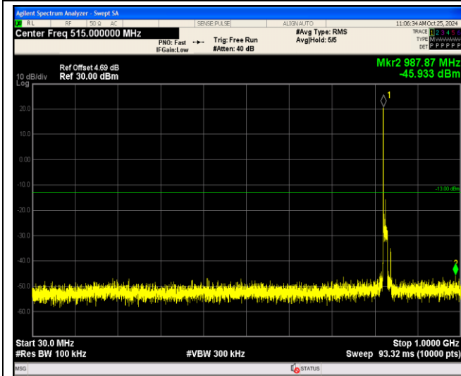
Band5-10MHz-16QAM-20525-1RB#0-Range1:30~1000MHz
