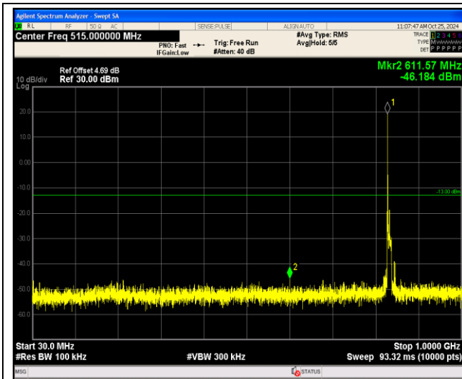
Band5-10MHz-64QAM-20600-1RB#0-Range1:30~1000MHz
