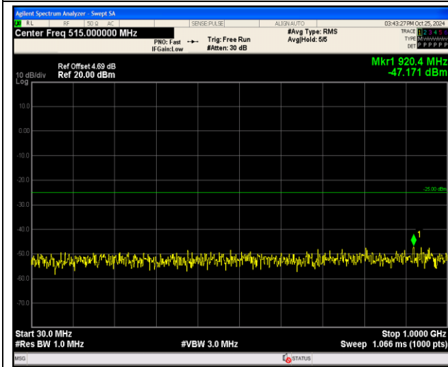
Band7-5MHz-16QAM-21425-1RB#0-Range1:30~100 0MHz
