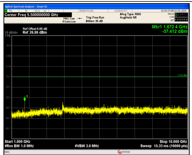
Band5-1.4MHz-QPSK-20643-1RB#0-Range2:1000~1 0000MHz
