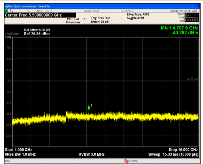
Band5-1.4MHz-64QAM-20525-1RB#0-Range2:1000~10000MHz
