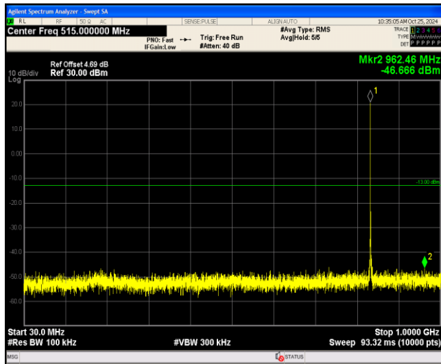
Band5-1.4MHz-64QAM-20643-1RB#0-Range1:30~1000MHz
