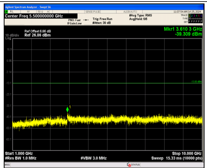
Band5-10MHz-64QAM-20600-1RB#0-Range2:1000~10000MHz
