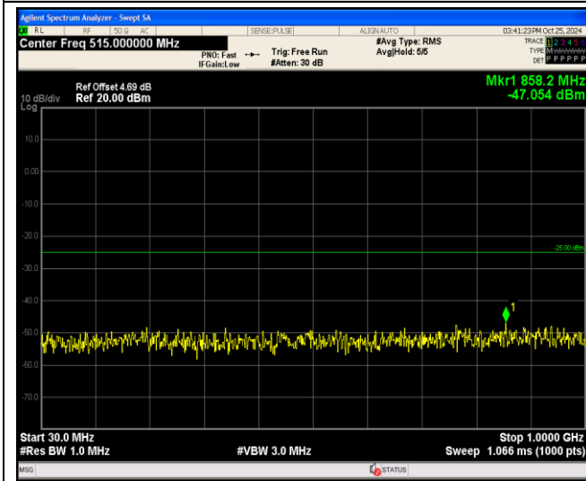
Band7-5MHz-QPSK-20775-1RB#0-Range1:30~1000MHz
