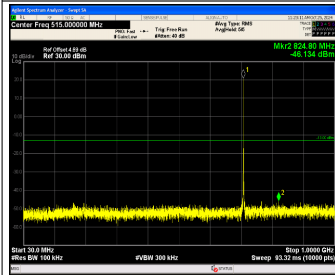
Band12-1.4MHz-QPSK-23173-1RB#0-Range1:30~1000MHz
