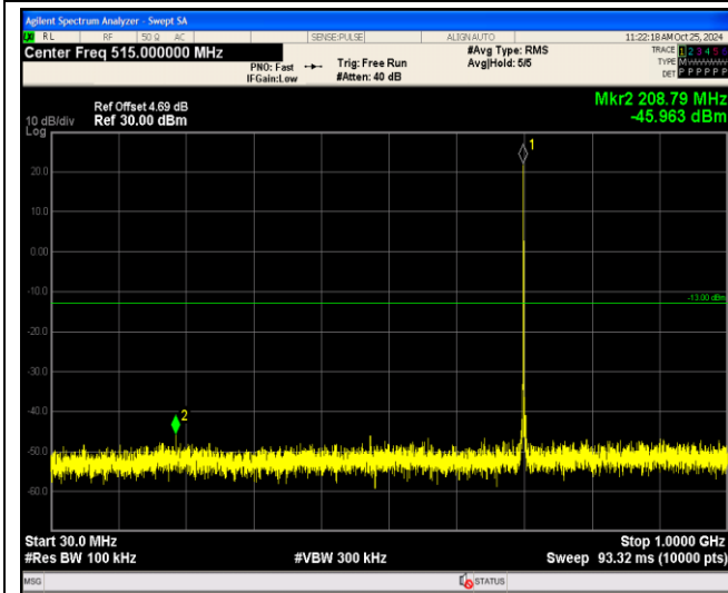
Band12-1.4MHz-QPSK-23173-1RB#0-Range1:30~1000MHz
