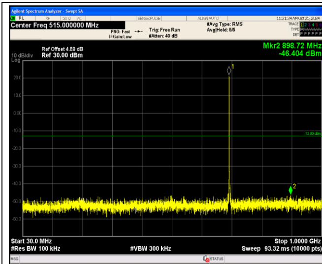
Band12-1.4MHz-QPSK-23095-1RB#0-Range1:30~1000MHz
