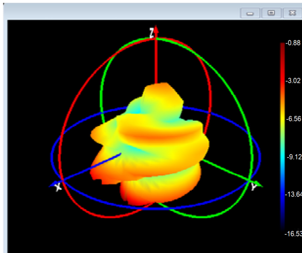
3D Radiation Pattern for 2450MHz
